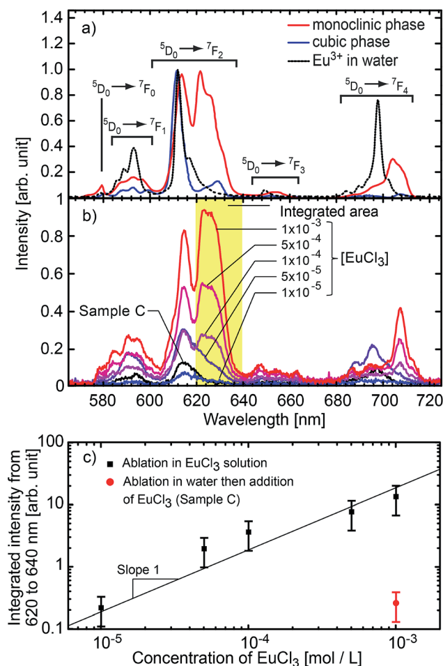
Fig. 4 (a) Luminescence spectra of reference Gd 2 O 3 :Eu mono- and cubic nanospheres, 62 cubic nanoplatelets, 63 and europium(III) chloride hexahydrate salt. (b) Luminescence spectra of the nanoparticles obtained by ablation of pure gadolinia in Eu 3+ solution at different concentrations. The black line corresponds to the reference sample C, i.e. undoped nanoparticles matured in a 10 -3 mol L -1 solution of EuCl 3 and then washed. The spectral resolution is 2 nm (FWHM). (c) Integrated signal between 620 nm and 640 nm for each concentration (monoclinic signature). The red dot corresponds to the signal from the reference sample C. The error bars correspond to the standard deviation of the amount of ablated material over 5 ablations. Solid line is a reading guide representing a linear power law.
