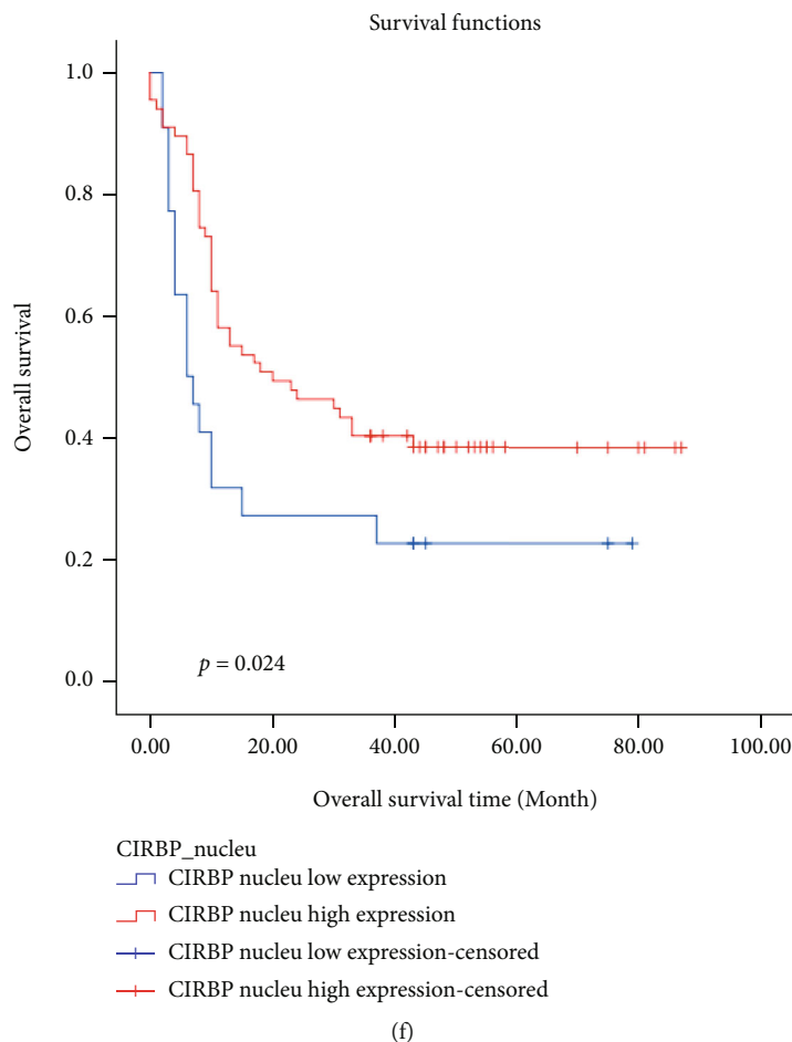
FIGURE 1: The expression level of CIRBP in pancreatic cancer. (a) The online database GEPIA2 showed the expression level of CIRBP in different tumors. (b) Data from database GEPIA2 showed the expression level of CIRBP in pancreatic cancer. (c) Survival curve analysis was performed using the expression data of CIRBP in database GEPIA2. (d) The expression level of CIRBP in the cytoplasm of cancer tissues was significantly lower than that of adjacent tissues. **** P < 0.0001 versus tumor. (e) The expression level of CIRBP in pancreatic cancer tissues was detected by immunohistochemistry. (f) Survival curve was analyzed according to the expression level of CIRBP in pancreatic cancer tissues.
