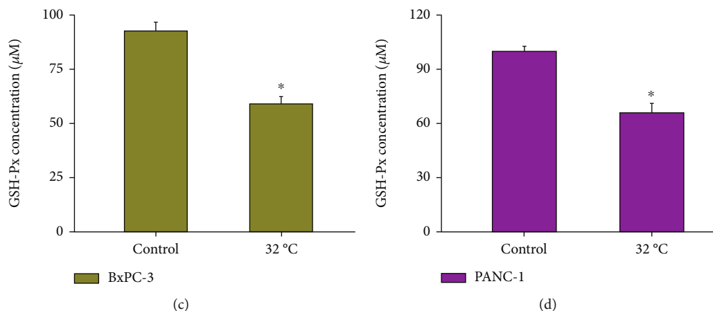
FIGURE 3: Cold induces \text{Fe}^{2+} accumulation and abnormal oxidative stress. BxPC-3 and PANC-1 cells were cultured at 37 (Control) or 32°C. (a) The increase in Prussian blue staining indicated an increase in \text{Fe}^{2+} accumulation level. (b) Representative confocal fluorescent images of MitoTracker™ Red FM (the mitochondrial indicator) and DCFH-DA (ROS indicator)-loaded cells. (c) GSH-Px activity was measured using a GSH-Px assay kit. * P < 0.05 versus Control.
