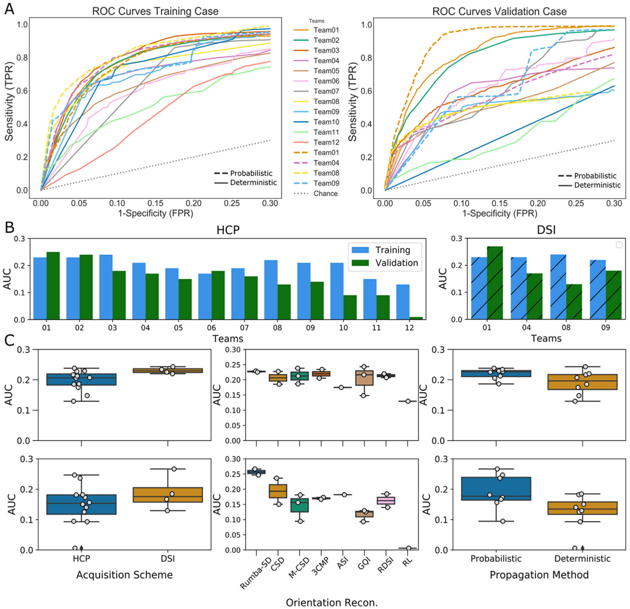
Fig. 2. Round 1 results.
