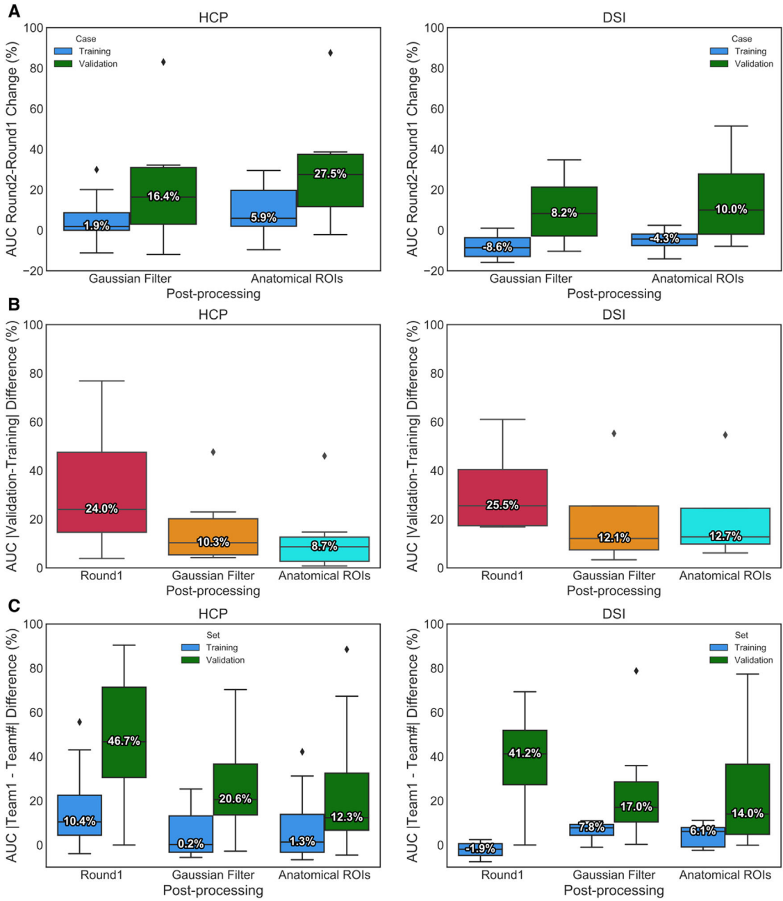
Fig. 4. Effect of harmonized pre- and post-processing.
