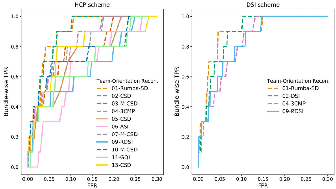
Fig. 5. Bundle-wise TPR.
