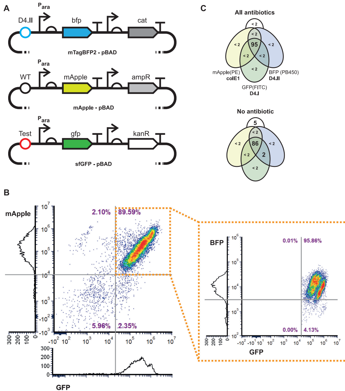
Figure 5. Selected plasmid origins intercompatibility. (A) pBAD vectors harbouring fluorescent protein genes (based on plasmids # 54519, #54536 and #54572 from Addgene) were engineered to harbour different replication origins and different selectable markers. (B) Flow cytometry analysis of bacteria harbouring colE1 , D4.I and D4.II origins after overnight growth in the absence of any antibiotic selection. Cells expressing both GFP and mApple are gated (orange box) and checked for BFP expression (inset dot plot). Histograms of individual channels (without gating) are shown. (C) Flow cytometry results are summarized in the Venn diagrams, showing all subsets above 2% of the population to the nearest percentage point. Rare combinations (below 2% of the total population) are shown as '<2' for clarity. Detection events without fluorescence (e.g. dead cells or residual electronic noise) are shown in the peripheral (white) set. For the colE1 , D4.I and D4.II combination, even in the absence of antibiotics, all plasmids remained stably in the cells in contrast to the two-plasmid cross-compatibility assays.
