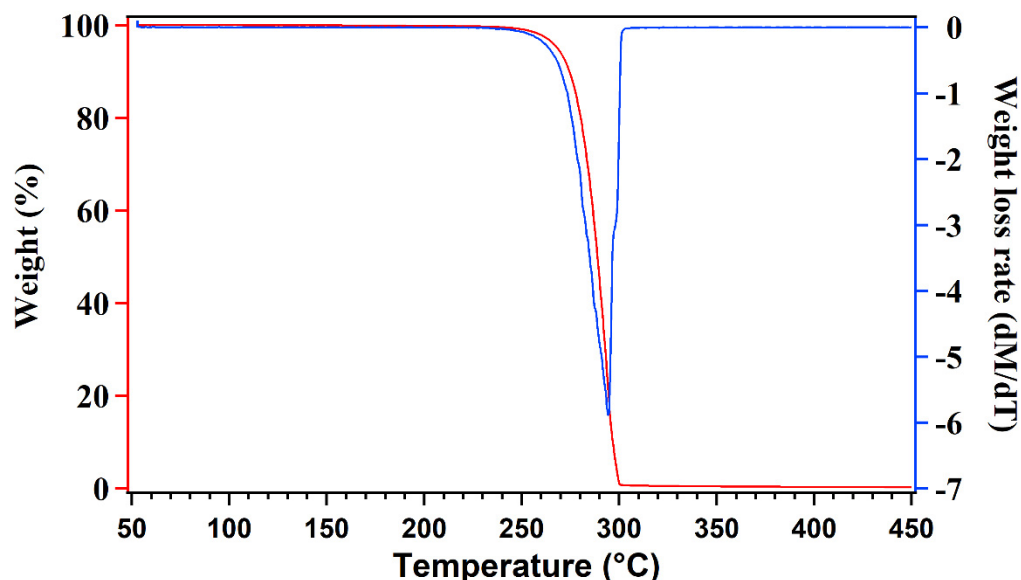
Figure 1. TGA (red) and DTG (blue) curves of P-0.
