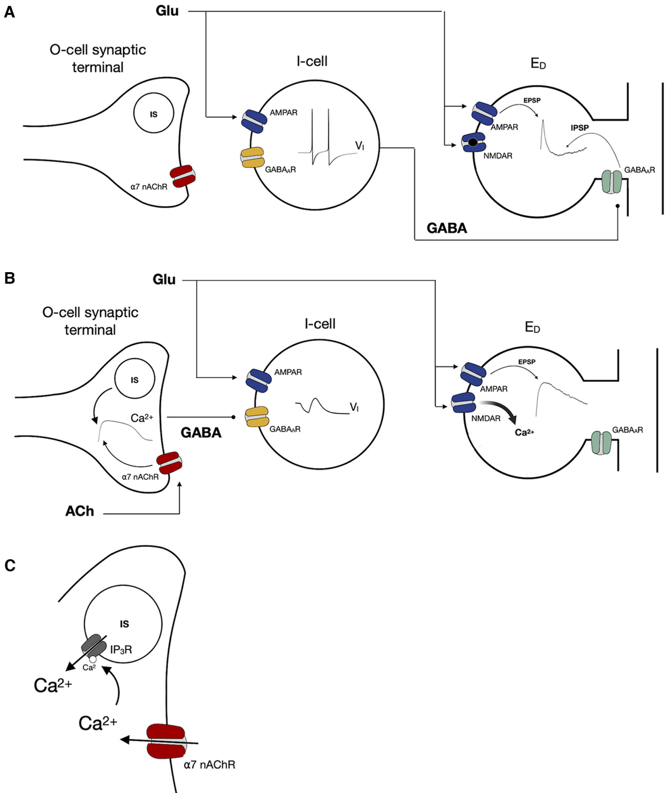
Figure 8. Scheme of the cholinergic and disinhibitory mechanisms that drive SC-CA1 potentiation. A , Glutamatergic activation of I-cells lead to spiking activity and consequent GABA release. Subsequently, glutamate inputs acting on E_D evoke an EPSP mediated by AMPAR immediately followed by an IPSP-mediated GABA acting on GABA A receptors. B , Cholinergic activation of \alpha 7 nAChR on OLM interneuron initiates a CICR process mediated by calcium internal stores (IS). This result in GABA release that inhibits the I-cell. The dendritic compartment does not receive GABAergic inhibition. The dendritic compartment can depolarize enough—and remain depolarized for long enough—to relieve Mg^{2+} block from NMDA receptors,
