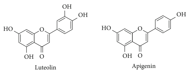
FIGURE 4: Chemical structures of luteolin and apigenin.
