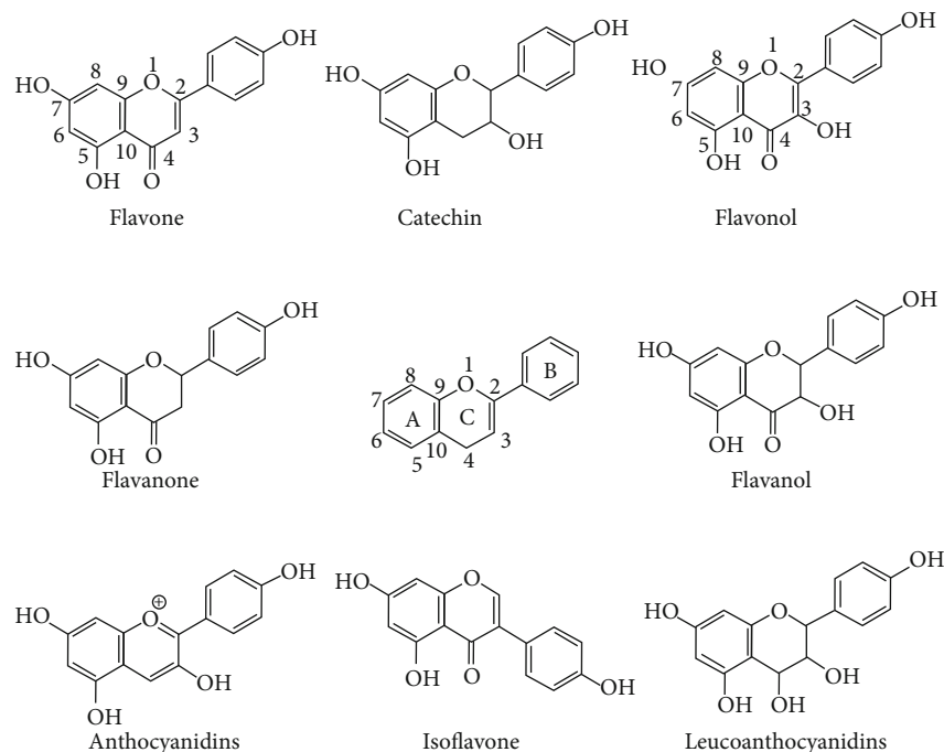
FIGURE 2: Chemical structures of some representative flavonoids and the basic skeleton of the flavonoids in the middle.
