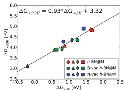
Fig. 6 (A) Scaling relation between \Delta G_{*OH} and \Delta G_{*OOH} for different studied h-BN@M complexes. (B) Volcano plot of ORR limiting potential as a function of \Delta G_{*OH} . Circle, triangle, diamond and square symbols indicate Ag, Cu, Pd and Pt supports, respectively.
