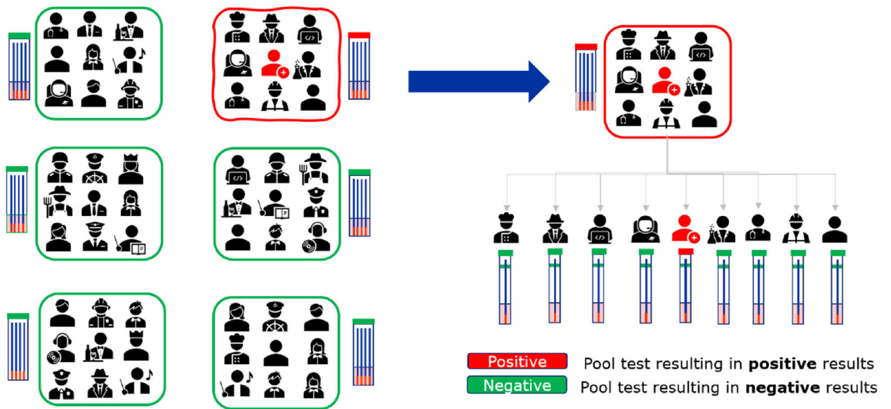
Fig. 1. Pool testing principle. Samples are pooled and each pool is tested. If a pool tests negative, as indicated in green, the test is complete. If the pool tests positive, as indicated in red, all samples of that pool are tested individually to identify the sample(s) that contributed to the positive pool.
