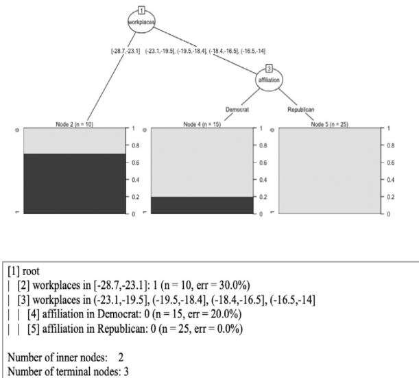
Fig. 4. CHAID dendrogram for Model 2.
