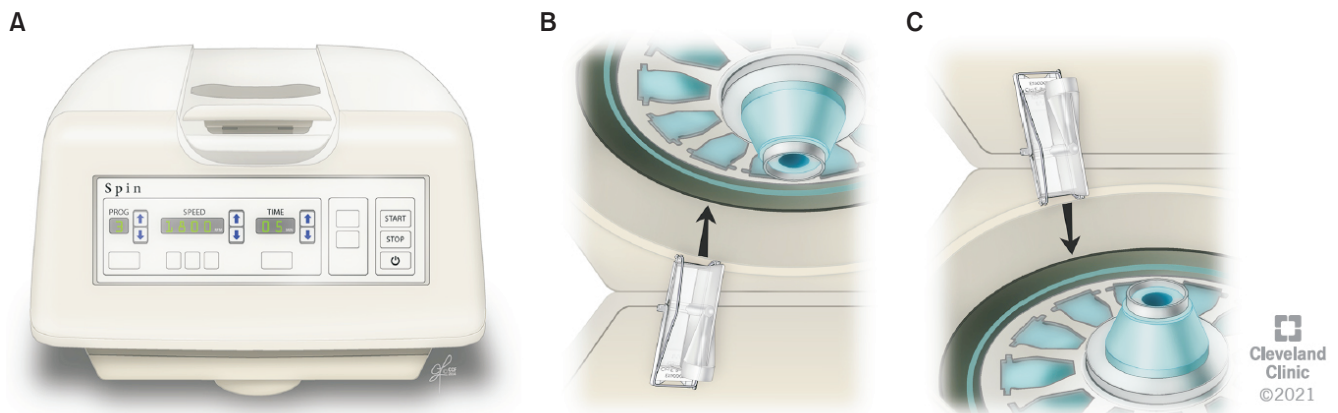
Fig. 2. (A) Cytospin and (B, C) inside view showing the special rotor for proper insertion of the Cytospin slide.
