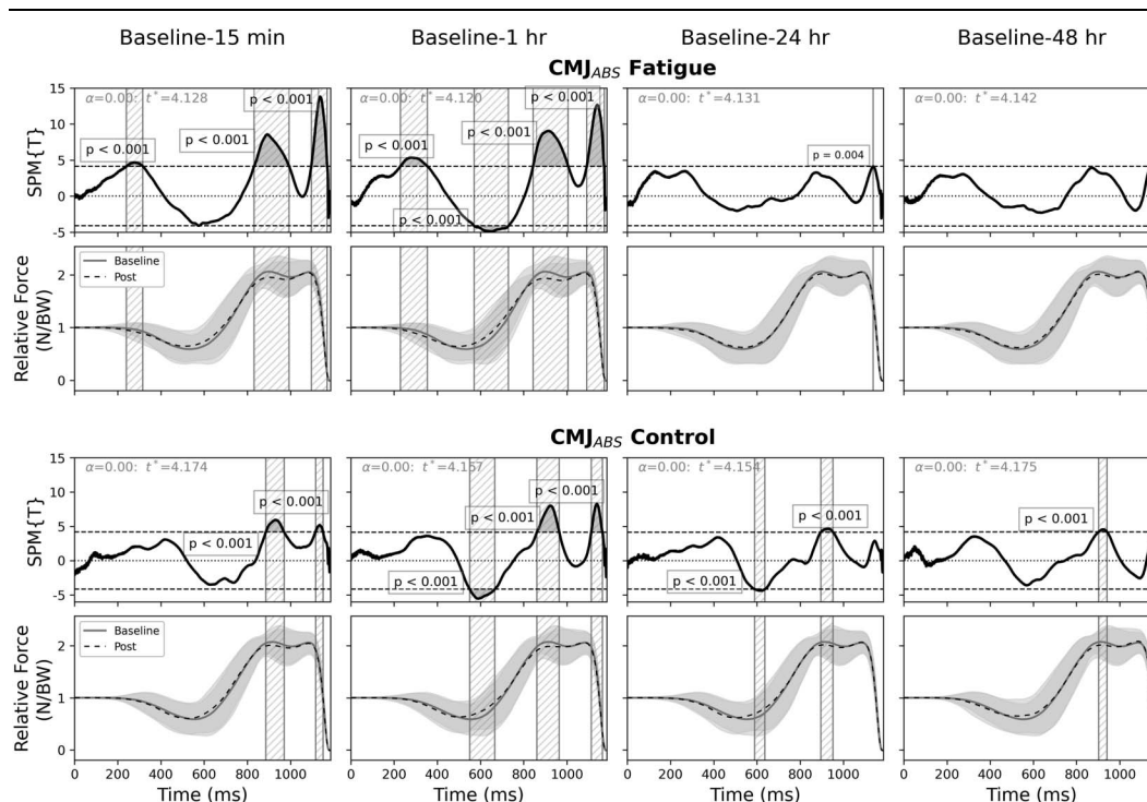
Figure 4. Follow-up SPM T-test with Bonferroni correction comparison between baseline and later time points in CMJ_{ABS} fatigue and control condition. Rows 1 and 3—Inference curves with suprathreshold clusters (shaded) and critical threshold (dashed line). Rows 2 and 4—CMJ mean force for baseline (solid line) and postcondition time points (dashed line) with SD cloud (shaded) standardized to body mass in newtons. CMJ = countermovement jump; SPM = statistical parametric mapping.
