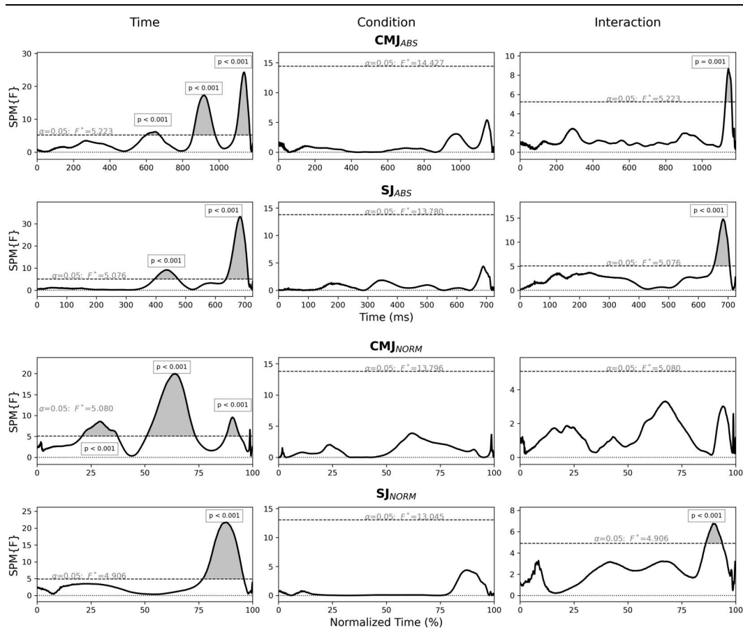
Figure 3. SPM 2-way repeated measures ANOVA results for CMJ_{ABS} , CMJ_{NORM} , SJ_{ABS} , and SJ_{NORM} as labeled. Inference curves with suprathreshold clusters (shaded) for time (column 1), condition (column 2), and interaction (column 3) with critical threshold (dashed line). ANOVA = analysis of variance; CMJ = countermovement jump; SJ = squat jump; SPM = statistical parametric mapping.
