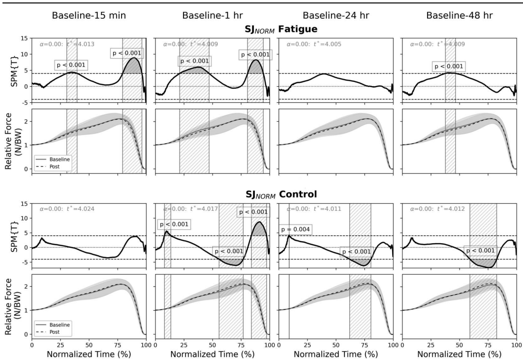
Figure 6. Follow-up SPM T-test with Bonferroni correction comparison between baseline and later time points in SJ_{NORM} fatigue and control condition. Rows 1 and 3—Inference curves with suprathreshold clusters (shaded) and critical threshold (dashed line). Rows 2 and 4—SJ mean force for baseline (solid line) and postcondition time points (dashed line) with SD cloud (shaded) standardized to body mass in newtons. SPM = statistical parametric mapping; SJ = squat jump.
