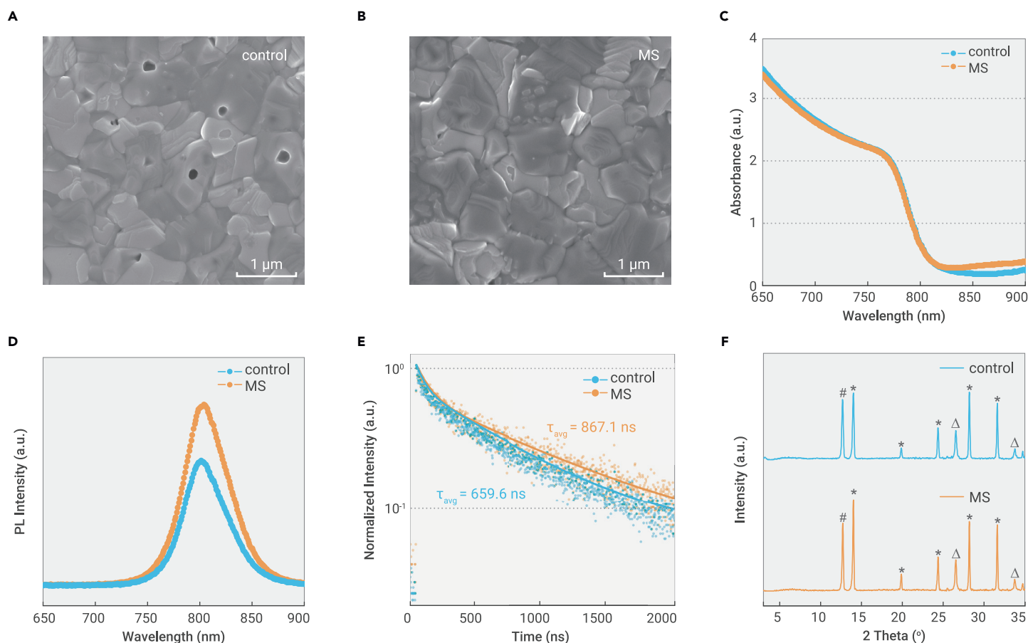
Figure 2. Perovskite thin film characterization (A–F) Scanning electron microscopy (SEM) images of top-view morphology (A and B), UV-vis spectra (C), static photoluminescence spectra (D), time-resolved photoluminescence decay (E), and X-ray diffraction pattern (F) of the control and MS-perovskite films (# denotes the PbI 2 phase, * denotes the FAPbI 3 perovskite phase, and Δ denotes the FTO substrate).
