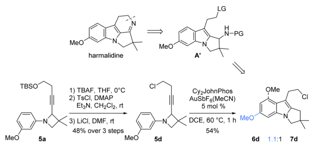
Scheme 8 Preparation of pyrrolo[1,2- a ]indole 6d for reverse cyclisation strategy.
