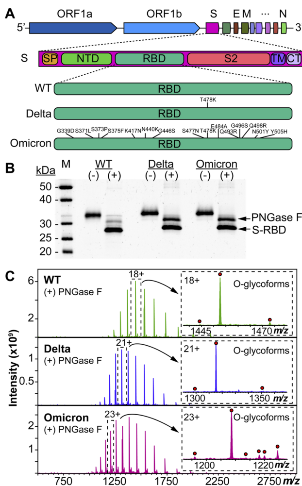
Fig. 1 Protein mutational mapping and high-resolution top-down MS of S-RBD arising from the WT, Delta, and Omicron variants. (A) Architecture of SARS-CoV-2 genome and illustration of the protein sequence changes for the S-RBD variants. (B) SDS-PAGE of the S-RBD variants before (–) and after (+) PNGase F treatment. Gel lanes were equally loaded (300 ng), and gel staining was visualized by SYPRO Ruby. (C) Raw MS1 of intact S-RBD proteoforms collected on the 12 T FTICR-MS after PNGase F treatment for the WT, Delta, and Omicron variants. All identified O -glycoforms are annotated in the inset with a red circle.
