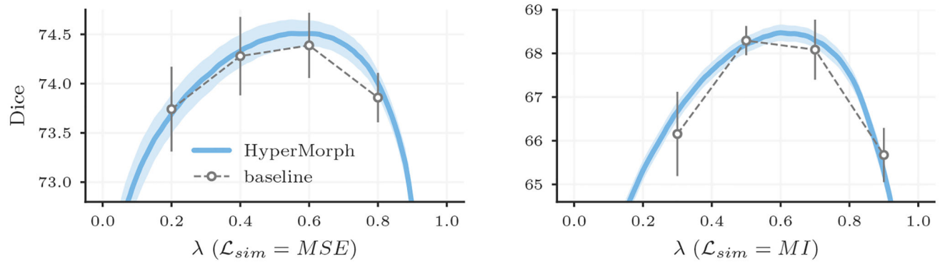
Figure 9: Variability across several training initializations for HyperMorph and baseline models. Error bars and fill regions span a 2- \sigma range around the mean registration accuracy, which is substantially tighter for HyperMorph.
