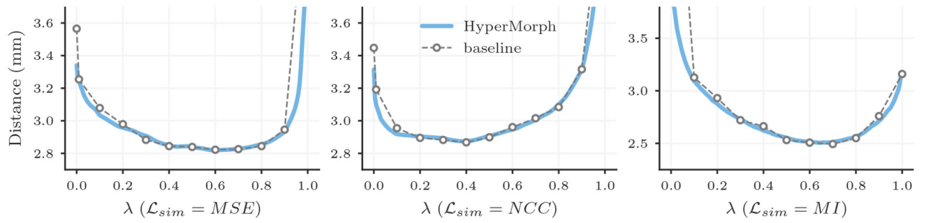
Figure 5: Mean 95th percentile surface distances achieved by a single HyperMorph model (blue) and baselines trained for different regularization weights \lambda (grey) when using MSE, NCC, or MI similarity metrics.
