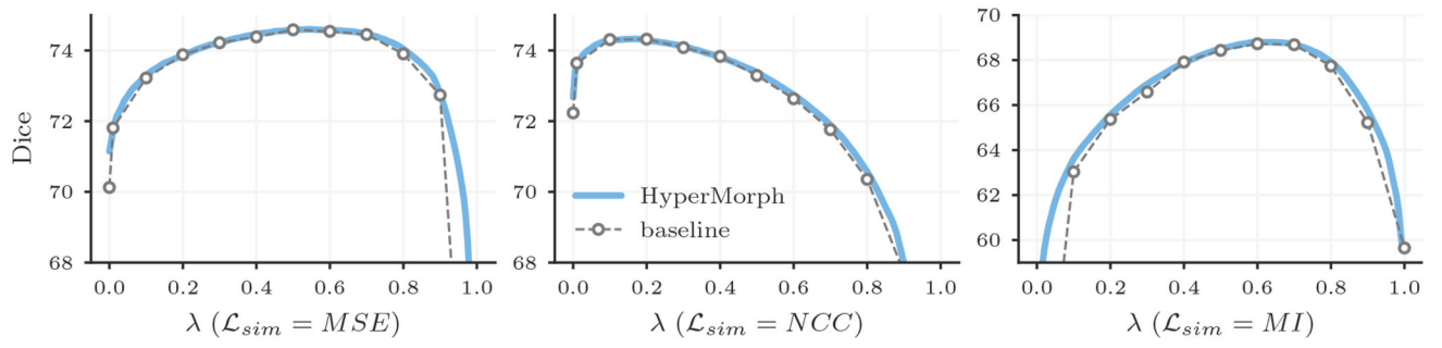
Figure 4: Mean Dice scores achieved by a single HyperMorph model (blue) and baselines trained for different regularization weights \lambda (grey) when using MSE, NCC, or MI similarity metrics.
