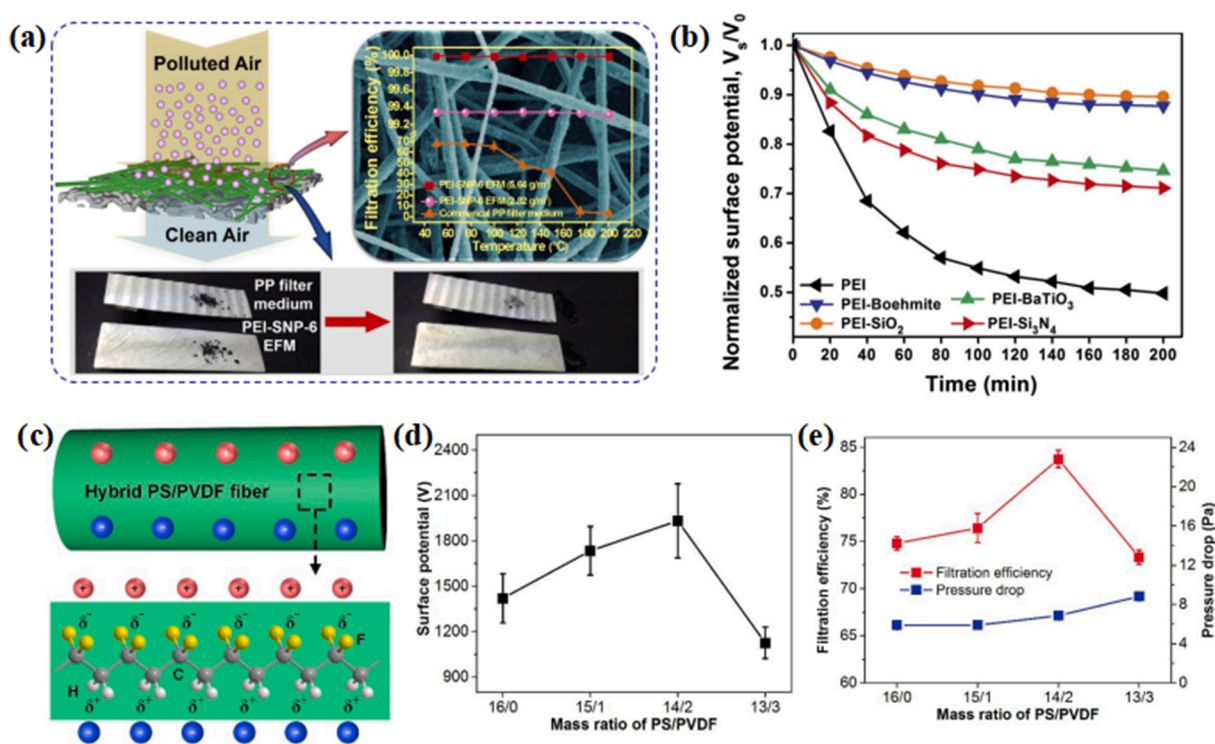
Fig. 4. (a) Schematic diagram of PEI/ \text{SiO}_2 nanofibrous membrane, and the filtration efficiency of different membranes under different temperatures. (b) Surface potential decay of different hybrid membranes at room temperature over time [83]. (c) Schematic illustrating the contribution of PVDF on electret effect. (d) Surface potentials of PS/PVDF electret fibers with different mass ratio. (e) Filtration efficiency and pressure drop of PS/PVDF membranes with different mass ratio [93].
