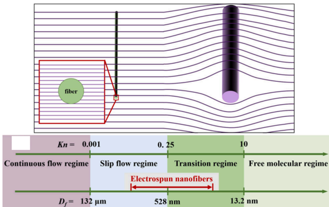
Fig. 2. Theoretical diagram of slip effect of single fiber. Where, K_n and D_f stands for Knudsen Number and the diameter of fibers, respectively [60].
