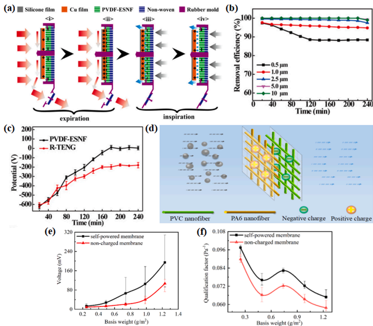
Fig. 6. (a) Working principles of the R-TENG by periodic expiration and inspiration. (b) The removal efficiency of R-TENG for particles with different diameters in 240 min durability test. (c) Average surface potential change of the single PVDF membrane and R-TENG in 240 min filtration [106]. (d) Schematic diagram for the air filtration process of the self-powered composite membrane. (e) The measured voltage on the two sides of the composite membranes of different combinations under airflow velocity of 0.1 m/s. (f) The QF of the composite membranes under airflow velocity of 0.1 m/s [107].
