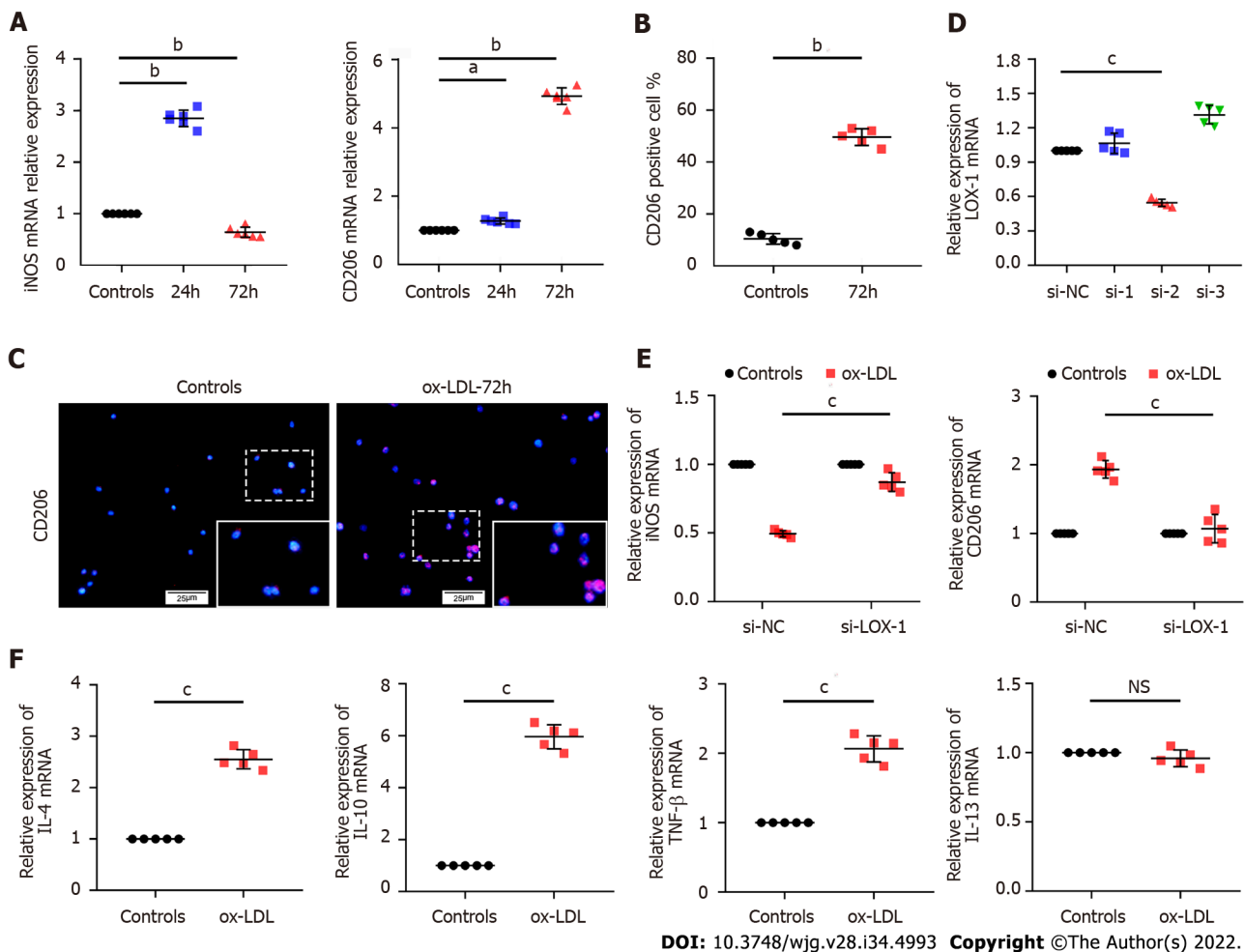
Figure 4 Continuous stimulation with oxidized low-density lipoprotein promotes CD206+ macrophages. A: Quantitative polymerase chain reaction (qPCR) detection of mRNA expression of CD206 and inducible nitric oxide synthase ( iNOS ) in THP-1 cells after oxidized low-density lipoprotein (ox-LDL) stimulation; B: Quantification of CD206-positive cells in RAW 264.7 cells based on IF results in Figure 4C; C: Cell fluorescence images of CD206 expression in RAW 264.7 cells after ox-LDL stimulation (scale bars represent 25 μm); D: qPCR detection of the expression of LOX-1 mRNA in THP-1 cells after transfection with LOX-1 small interfering RNA of different sequences; E: qPCR detection of the expression of iNOS and CD206 mRNA in THP-1 cells with low expression of LOX-1 stimulated with ox-LDL; F: qPCR detection of the expression of interleukin IL-4 , IL-10 , IL-13 , and tumor necrosis factor-β mRNA in THP-1 cells after 72 h of ox-LDL stimulation. Data are shown as the mean ± SD. Statistical analyses were conducted using an unpaired t test (Figure 4A, 4D, 4E, and 4F) or one-way analysis of variance followed by Dunnett's multiple comparison test (Figure 4B). The boxed area is enlarged in the bottom right corner. a P < 0.05, b P < 0.01, c P < 0.001. ox-LDL: Oxidized low-density lipoprotein; iNOS : Inducible nitric oxide synthase; IL : Interleukin; TNF : Tumor necrosis factor; si-NC: Small interfering RNA negative control.
