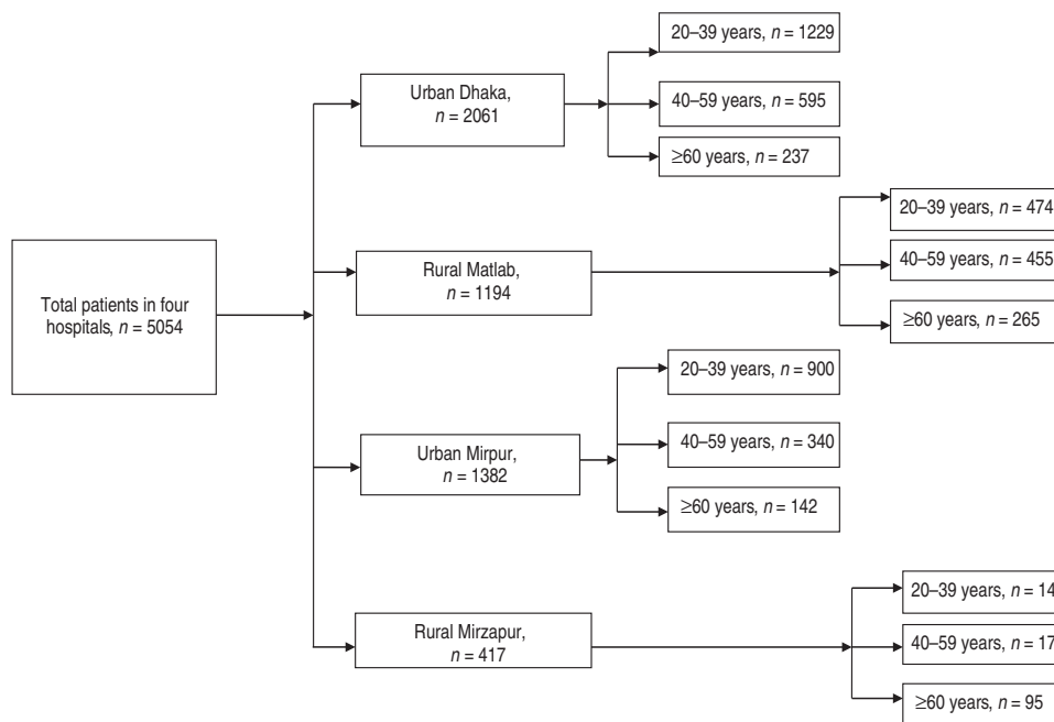
Fig. 1. Sampling frame.
