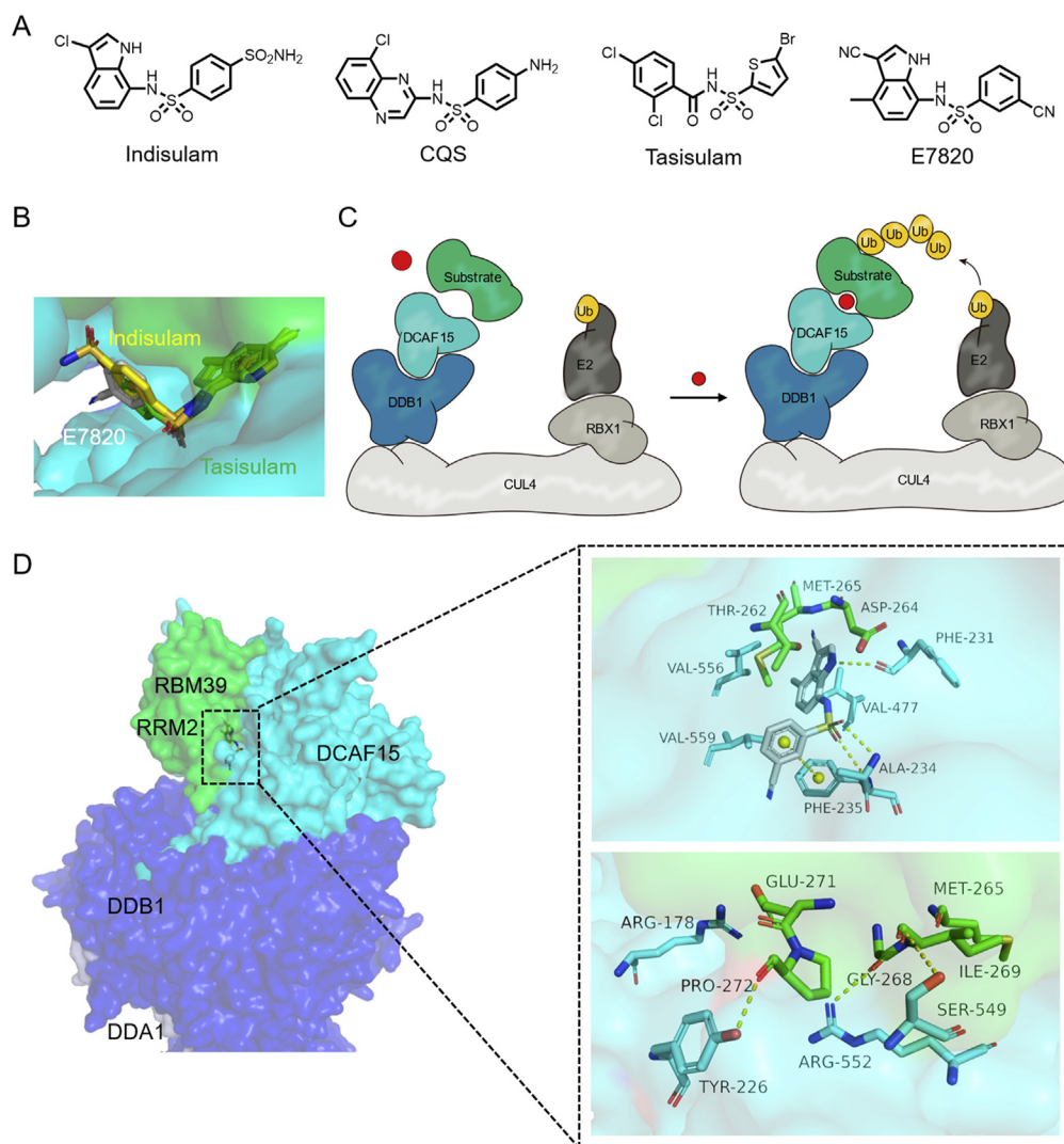
Figure 8 (A) Chemical structures of aryl-sulfonamides molecular glues. (B) A combination of E7820 and indisulam on the surface of DCAF15 and RBM39 (indisulam PDB:6Q0W). (C) Schematic diagram of the action mechanism of aryl sulfonamides molecular glues. (D) DDB1-DCAF15-E7820-RBM39 co-crystal structure (DDB1 colored in blue, DCAF15 colored in cyan, RBM39 colored in green, DDA1 colored in lightblue; PDB:6Q0R). Hydrogen bonds are shown as yellow dotted lines.
