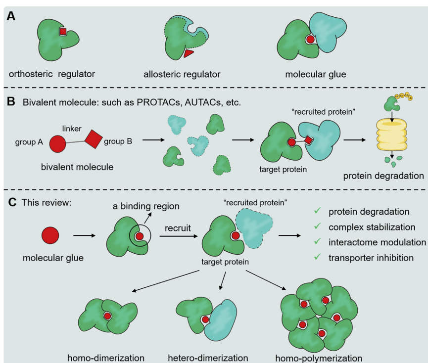
Figure 1 (A) Difference of orthosteric regulator, allosteric regulator and molecular glue. (B) Schematic diagram of divalent molecular interaction mode. (C) Schematic diagram of molecular interaction mode and classification of protein polymerization patterns induced by molecular glues.
