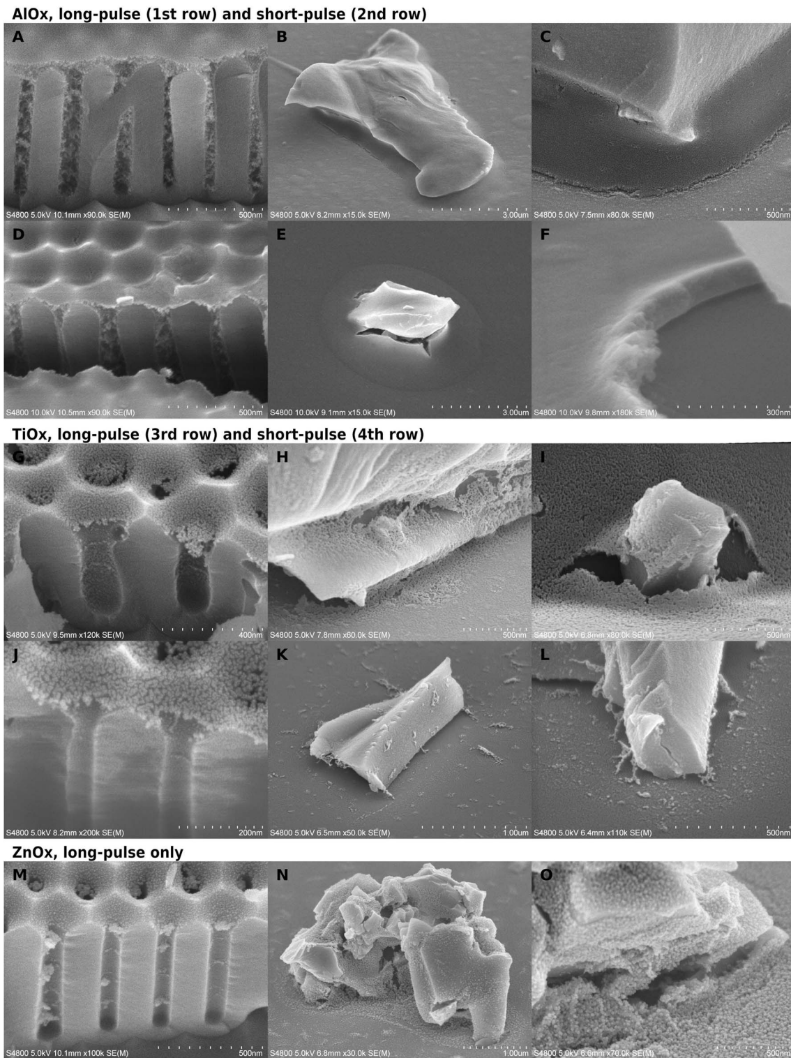
Fig. 2 SEM micrographs of calcined VPI experiments on AAO (first column) and glass (second and third columns) substrates with either one cycle of long pulses or 10 cycles with short pulses. (A–C) Alumina with long pulses. (D–F) Alumina with short pulses. (G–I) Titania with long pulses. (J–L) Titania with short pulses. (M–O) Zinc oxide with long pulses.
