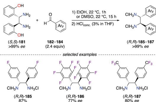
Scheme 20 Stereospecific preparation of C 2 -symmetric fluorinated DPEN ligands.
