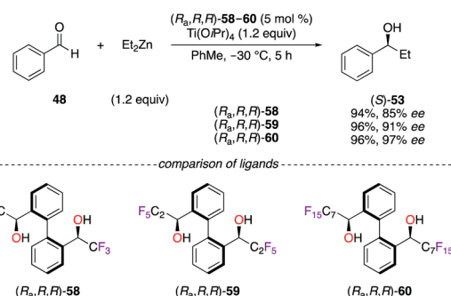
Scheme 7 Ti IV -Catalyzed ethylation reaction using \alpha,\alpha' -C n F n+1 -diol ligands.
