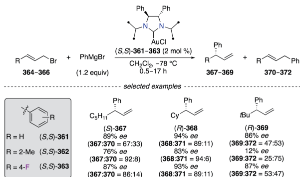
Scheme 38 NHC-Cu I -Catalyzed AAr reaction of aliphatic allylic bromides with phenyl magnesium bromide.
