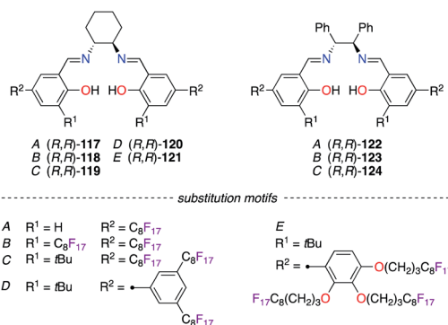
Fig. 6 Salen ligands bearing fluorinated motifs.
