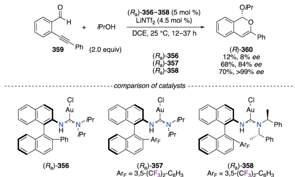
Scheme 37 Au I -Catalyzed cyclization of 359 into ( R )-360.
