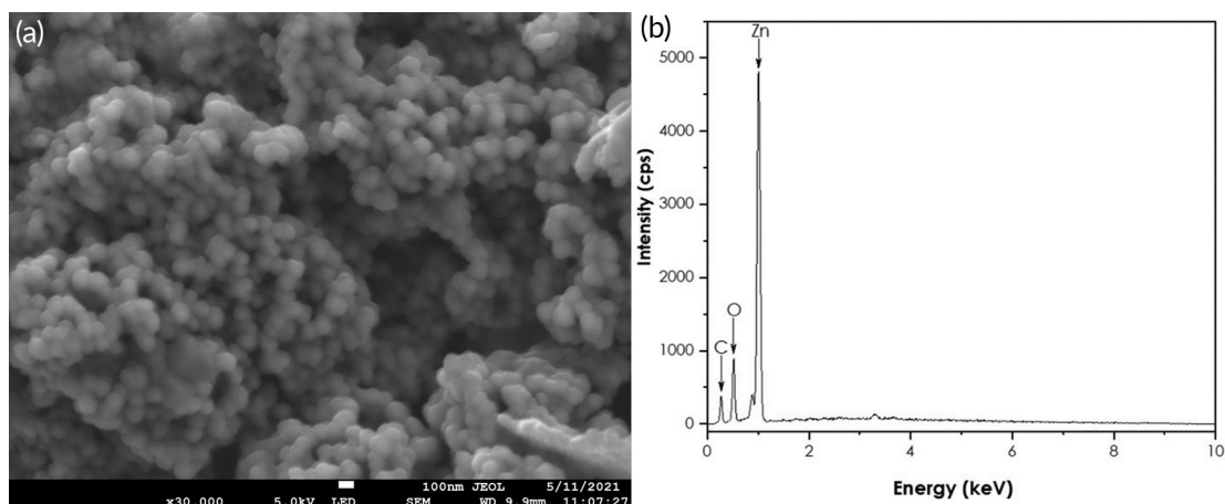
Figure 8. (a) Scanning electron microscopy image and (b) Energy-dispersive X-ray spectra of ZnO nanoparticles.
