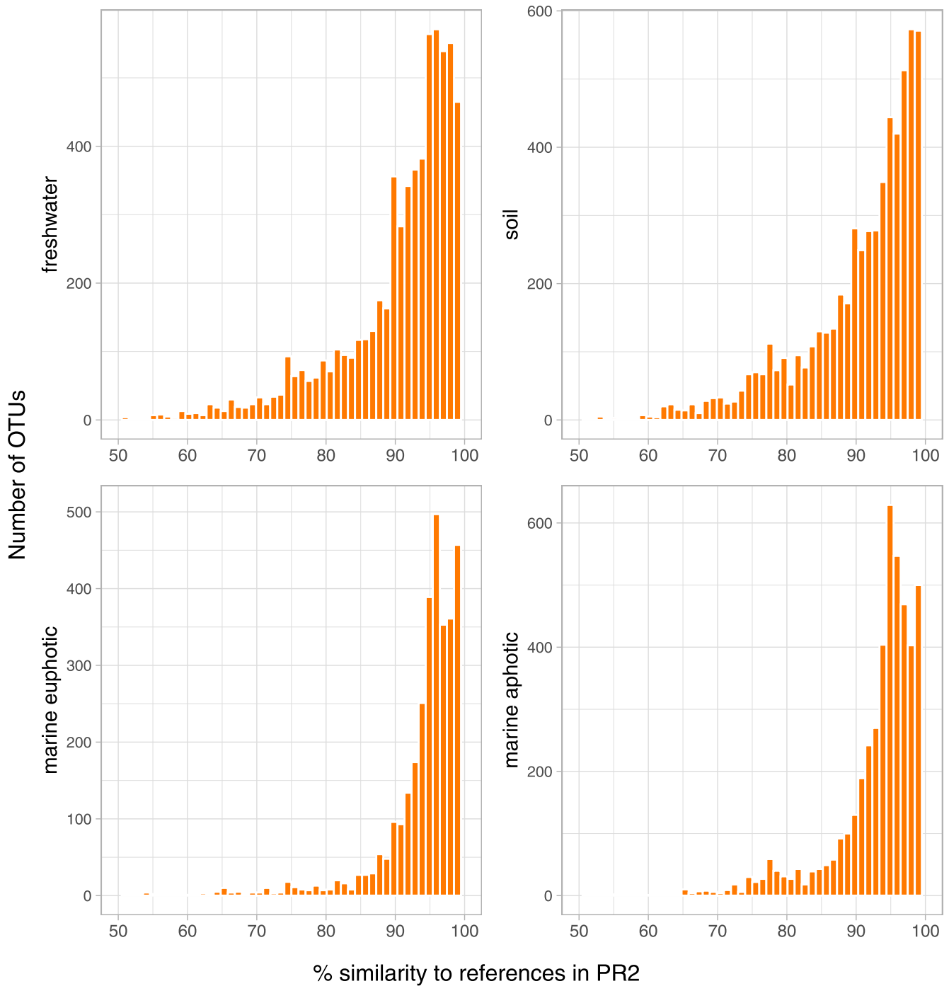
Extended Data Fig. 3 | Percentage similarity of OTUs to references in PR 2 . Percentage similarity of OTUs (18S sequence only) against reference sequences in the PR 2 database 30 , as determined by vsearch global search 91 . All sequences (OTU queries and references) were trimmed with primers 3NDF and 1510 R so that they spanned the same region.
