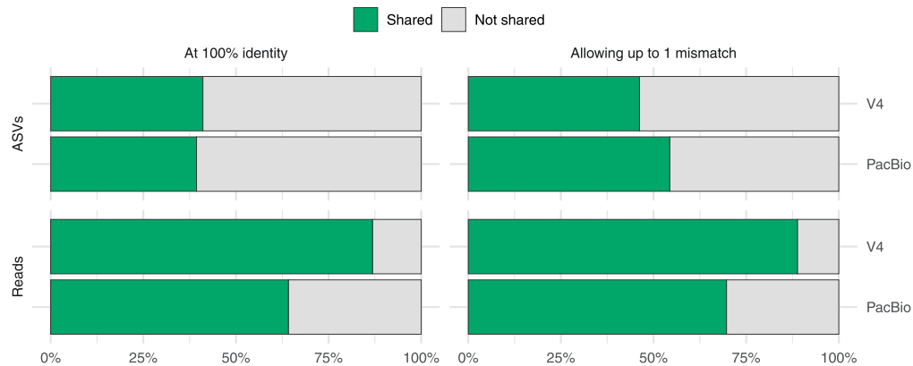
Extended Data Fig. 1 | Shared ASVs between PacBio and Illumina sequencing. Comparison of PacBio and Illumina sequencing. PacBio amplicons were compared with metagenomes (mTags), V4 amplicons, and V9 amplicons from three marine samples corresponding to the pico size fraction from the Malaspina expedition 27 . Station 76|Surface did not have V9 amplicon data. ASVs = Amplicon Sequence Variants. (a) Number of reads and ASVs for each sample for each marker. The mTags represent sequence length of ca. 100 bp, so no ASV level is available, as this short length does not give enough resolution. More PacBio sequences were generated for each sample compared to Illumina sequences. (b) Comparison of PacBio ASVs (that is de-noised, preclustered sequences) with the ones given by V4 amplicons. A similar comparison with V9 ASVs was not carried out as not all samples had V9 Illumina data available. Around half of the sequences were shared, which represented the majority of reads.
