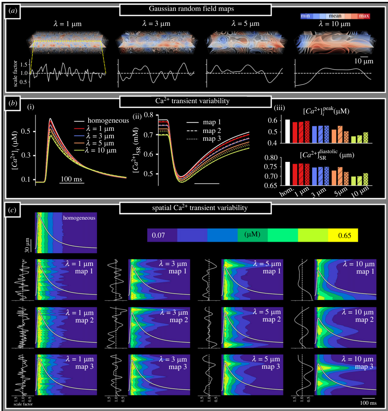
Figure 3. Ca 2+ transient variability as a consequence of SERCA2a heterogeneity. (a) Illustration of the GRF maps, describing the local J_{\text{up}}^{\text{max}} scale factor, produced at different length-scales (upper). The value of the scale factor along a longitudinal linescan through the centre of the cell is shown for clarity (lower). Maps shown correspond to ‘map 1’ of the three independent GRF maps used at each length-scale. (b) Whole-cell Ca 2+ transients (i) and SR-Ca 2+ (ii) during normal pacing, for homogeneous control (white) and heterogeneous SERCA2a maps at each length-scale (1 \mu\text{m} —red; 3 \mu\text{m} —blue; 5 \mu\text{m} —orange; 10 \mu\text{m} —yellow); three maps at each length-scale were used (solid, dashed and dotted lines). Summary of the CaT magnitude (iii) and diastolic SR-Ca 2+ (iv) at each length-scale and for each map. (c) Space–time images of the Ca 2+ transient in the longitudinal axis (through the centre of the cell) in the homogeneous and all heterogeneous map conditions, corresponding to the same normal pacing excitations as shown in (b). Normalized whole-cell-average CaTs are overlaid in white for context. Plots to the left of each space–time image show the SERCA2a scale factor along the same longitudinal linescan (as illustrated in (a)).
