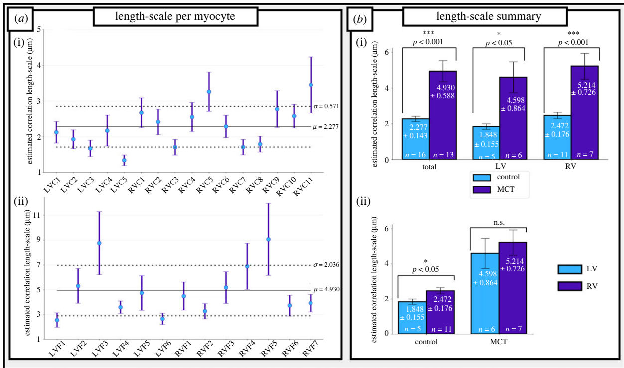
Figure 2. SERCA2a heterogeneity in control and RV-HF cardiomyocytes. (a) The comparison of cell-average correlation length-scales, \lambda , in control (saline-treated) (i) cells and monocrotaline (MCT)-treated cells (ii). Horizontal lines represent overall mean (full line) and s.d. (dotted line) for control and MCT cells, respectively. Vertical error lines are 95% confidence intervals. (b) Comparison of mean \lambda in control and MCT-treated rat ventricular myocytes (i) and in left ventricular (LV) and right ventricular (RV) cells (ii). (Online version in colour.)
