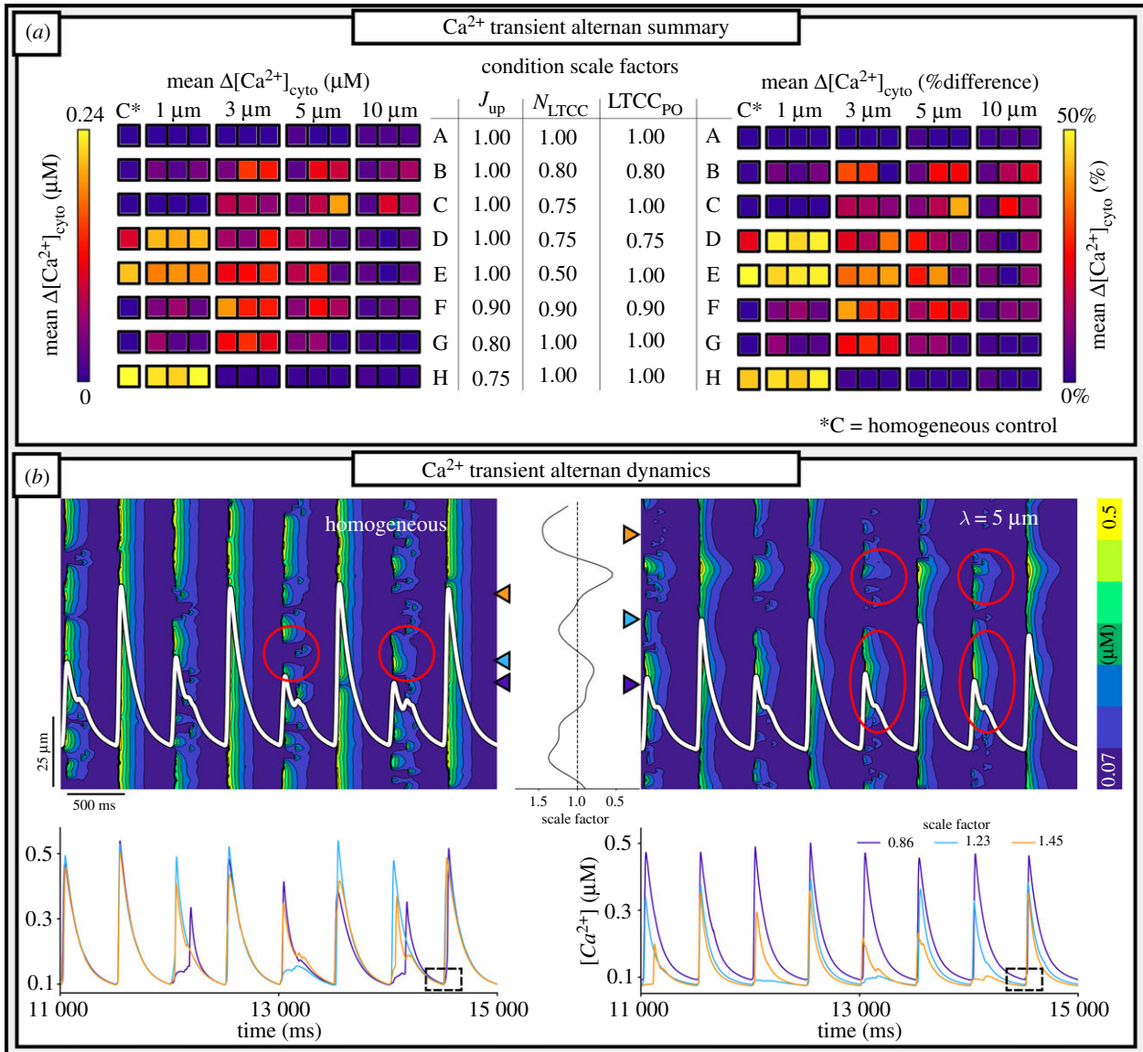
Figure 5. Summary of alternans behaviour in control to pro-arrhythmic conditions. (a) Colourmaps detailing the mean beat-to-beat difference in cytosolic Ca 2+ (left) and percentage difference (right) in a range of conditions from control (a) to pro-arrhythmic (b–h) at 120 bpm. Conditions are described by scaling factors applied to each of J_{\text{up}}^{\text{max}} (whole-cell SERCA2a flux), N_{\text{LTCC}} (L-type-Ca 2+ channel density) and \text{LTCC}_{\text{PO}} (channel opening transition rate). Maps are organized left to right. (b) Space–time plots showing CaT alternans in two different conditions (upper). Whole-cell CaT is overlaid in white for context. Circled regions illustrate those which show either different behaviour on a beat-to-beat basis for the small beat (homogeneous, (i)) or broadly the same behaviour for the small beat (heterogeneous, (ii)). Lower panels show the local CaT at three selected CRUs for the same two conditions; coloured triangular markers indicate the location of each CRU selected for the plot. In the heterogeneous condition, each CRU has its own corresponding J_{\text{up}}^{\text{max}} scale factor, indicated by the colour key. The dotted square highlights the same diastolic Ca 2+ in the homogeneous condition and different diastolic Ca 2+ in the heterogeneous condition.
