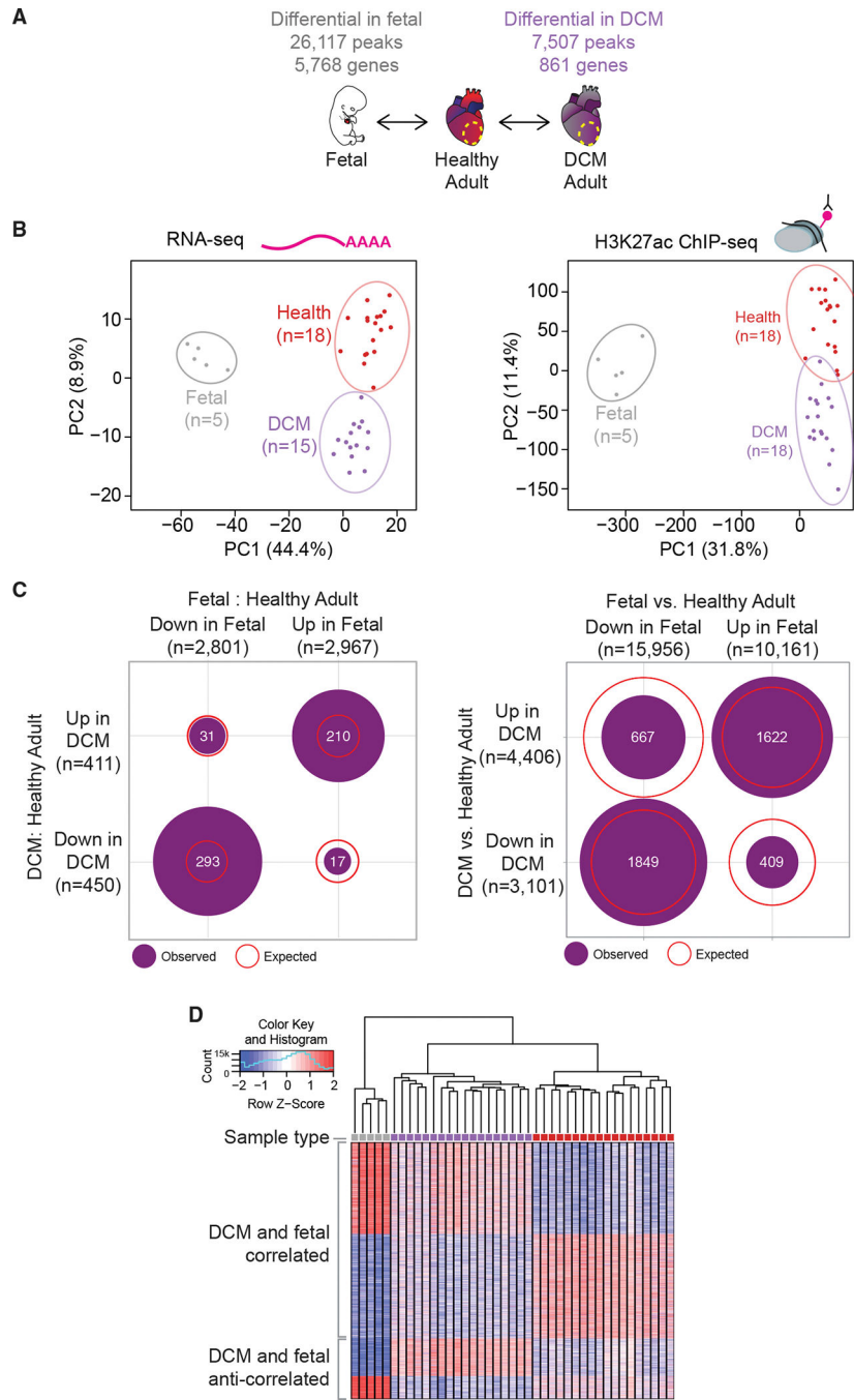
Figure 5. Fetalization is a driver of regulatory change in heart disease (A) Schematic of experimental comparisons and number of differential genes/peaks. (B) Principal-component analysis showing the first two principal components (PC1 and PC2) for the top 1,000 variably expressed genes from RNA-seq (left) and for distal enhancer peaks from ChIP-seq (right). Prenatal samples are gray, DCM samples are purple, and healthy samples are red.
