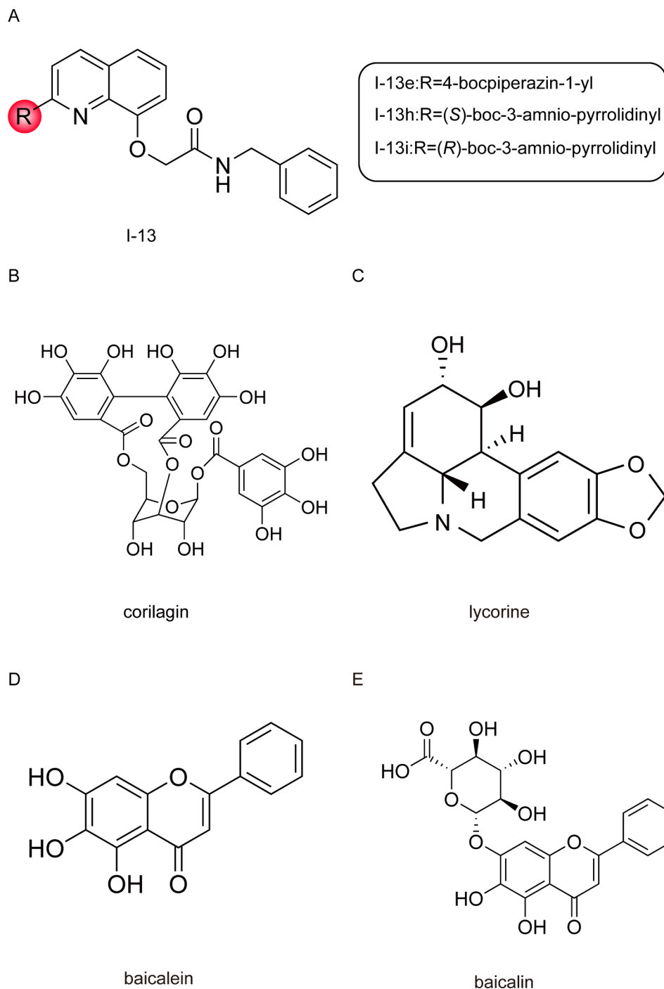
Fig. 9. Structures of non-nucleoside inhibitors.
