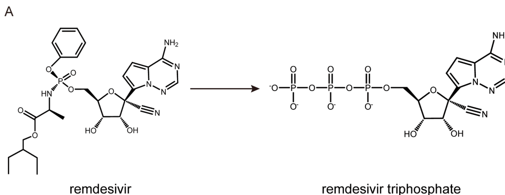
Fig. 3. Cryo-EM structure of remdesivir bound to the RdRp complex of SARS-CoV-2 (PDB ID:7BV2). (A) Chemical structures of remdesivir and remdesivir triphosphate. (B) Overall view of nsp12-nsp7-nsp8 in complex with template-primer RNA and remdesivir monophosphate (RDV-MP) and close-up view of the interactions between the SARS-CoV-2 RdRp active site and remdesivir. The potential polar contacts are shown as yellow dashed lines. The protein and RNA are shown in cartoons with the key residues involved in remdesivir interaction shown in lines and labeled in black and red, respectively. The RDV-MP is shown as a stick model.
