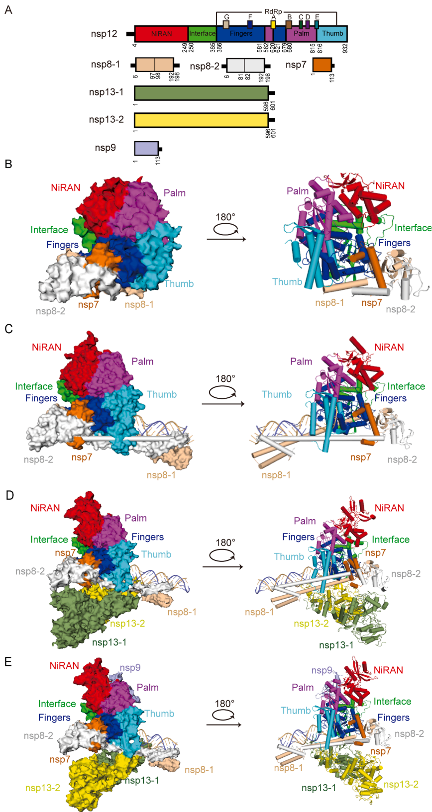
Fig. 2. Structure of SARS-CoV-2 replication-transcription complex (RTC) (A) The schematic diagram for the domain organization of each component in the RTC, containing nsp12, nsp7, two copies of nsp8 (nsp8-1 and nsp8-2), two copies of nsp13 (nsp13-1 and nsp13-2) and nsp9. The interdomain borders are labeled with residue numbers. In nsp12, the conserved sequence motifs A-G are depicted. The components and domains are colored as follows: nsp12 NiRAN, red; nsp12 Interface, green; nsp12 Fingers, blue; nsp12 Palm, magenta; nsp12 Thumb, cyan; nsp7, orange; nsp8-1, wheat; nsp8-2, white; nsp13-1, split-pea; nsp13-2, yellow; nsp9, light blue. The color coding corresponds to the figures throughout this manuscript. (B) Cryo-EM densities (left) and cartoon representations (right) of SARS-CoV-2 apo RdRp complex (nsp7-nsp8 2 -nsp12) in different views (PDB ID:7BW4). (C) Cryo-EM densities (left) and cartoon representations (right) of SARS-CoV-2 polymerase in complexes with RNA (nsp7-nsp8 2 -nsp12-RNA, central RTC) in different views (PDB ID:6YYT). The RNA is depicted with the template strand in slate and the primer/product strand in light orange. (D) Cryo-EM densities (left) and cartoon representations (right) of SARS-CoV-2 central RTC with nsp13 helicases (nsp7-nsp8 2 -nsp12-nsp13 2 -RNA, elongation RTC) in different views (PDB ID:6XEZ). (E) Cryo-EM densities (left) and cartoon representations (right) of SARS-CoV-2 elongation RTC with nsp9 (nsp7-nsp8 2 -nsp12-nsp13 2 -nsp9-RNA, extended E-RTC) in different views (PDB ID:7CYQ). Nsp9 binds to the catalytic center of the nsp12 (RdRp) NiRAN domain.
