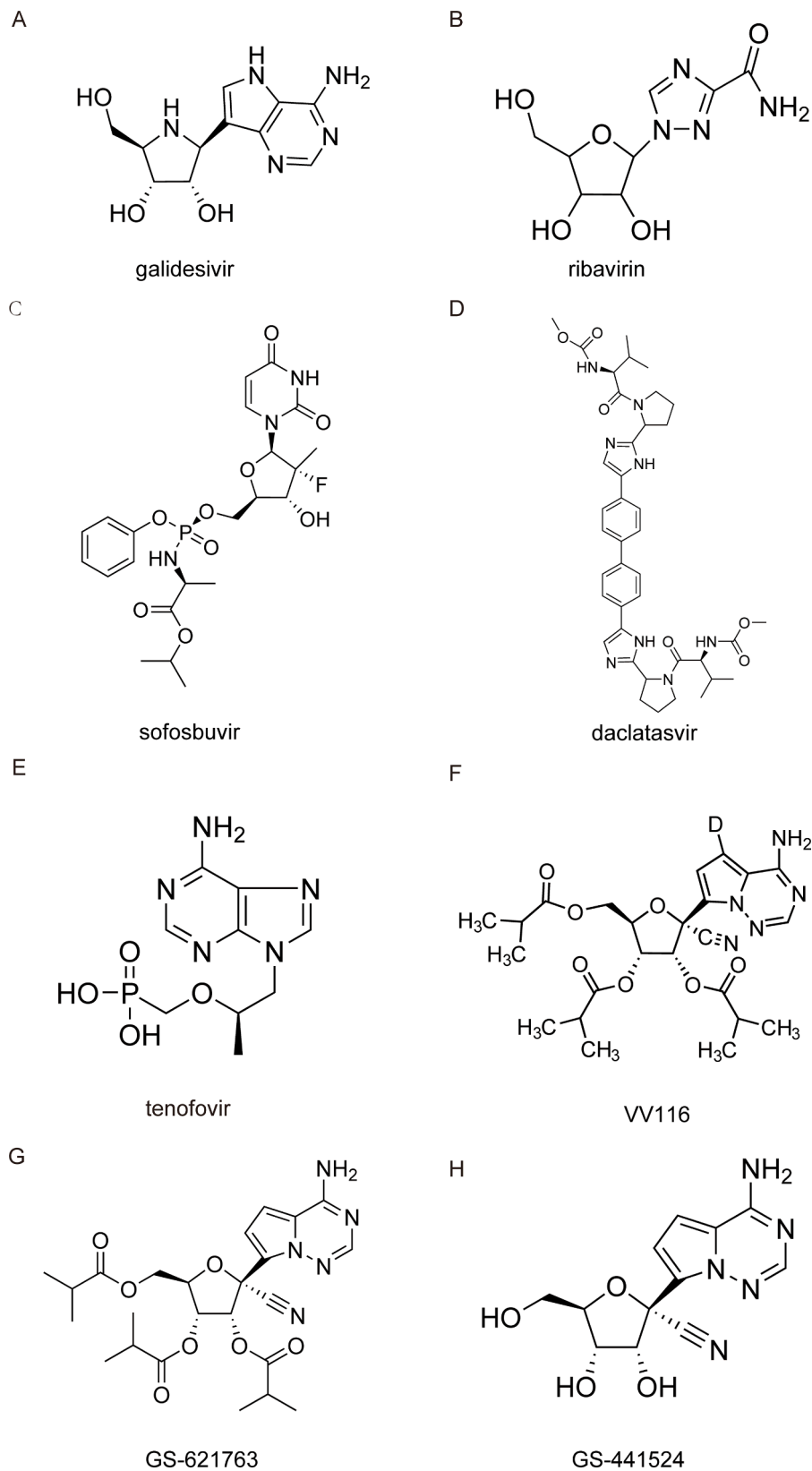
Fig. 6. Structures of nucleoside analog inhibitors.
