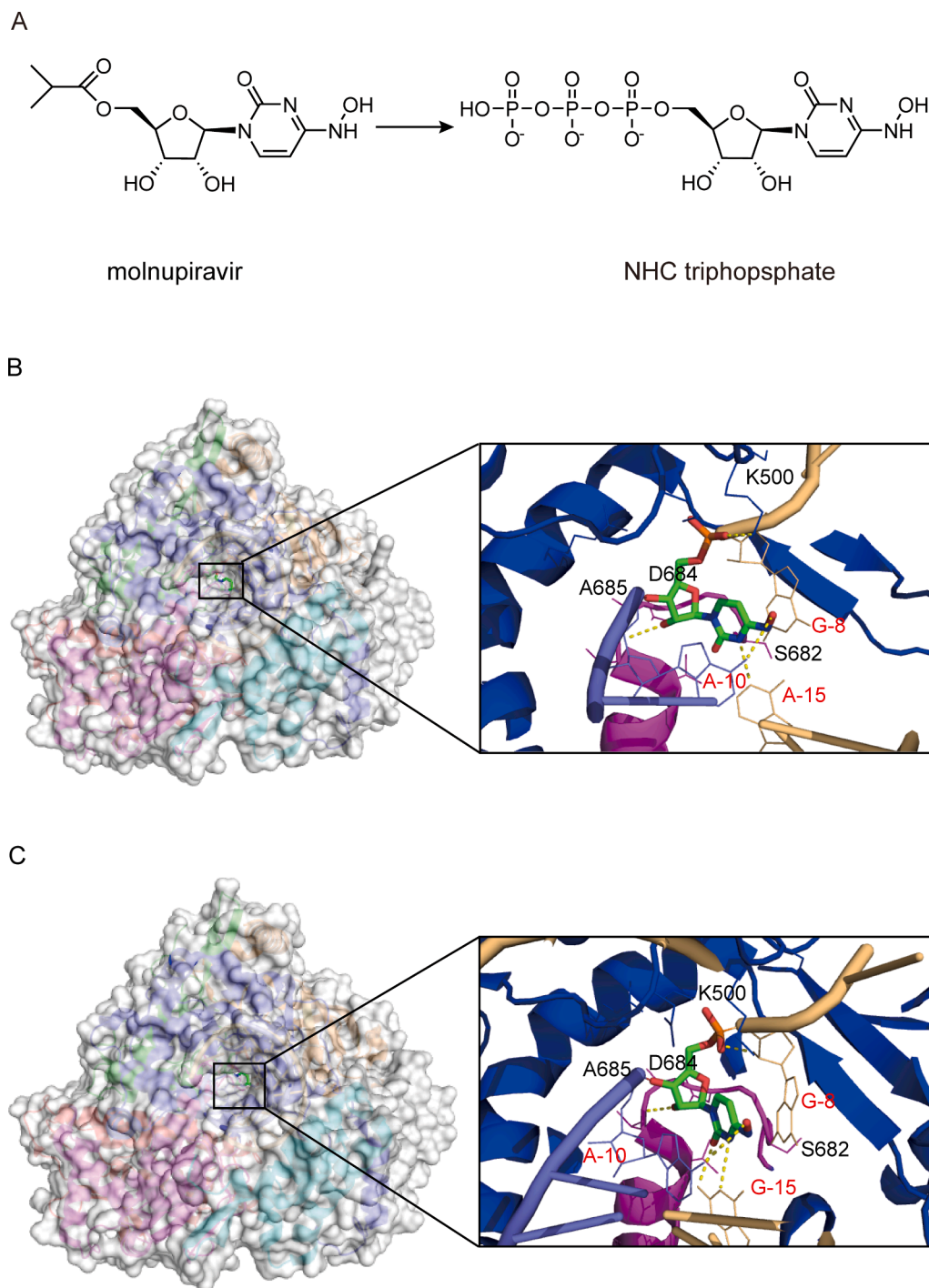
Fig. 5. Cryo-EM structure of NHC bound to the RdRp complex of SARS-CoV-2. (A) Chemical structures of molnupiravir and NHC triphosphate. (B and C) Overview of RdRp-RNA structure with an NHC monophosphate in the RNA template strand and close-up views of the interactions between the SARS-CoV-2 RdRp active site and NHC base paired to A(B) (PDB ID:7OZU) and base paired to G(C) (PDB ID:7OZV). The potential polar contacts are shown as yellow dashed lines. The protein and RNA are shown in cartoons with the key residues involved in NHC interaction shown in lines and labeled in black and red, respectively. The NHC are shown as stick models.
