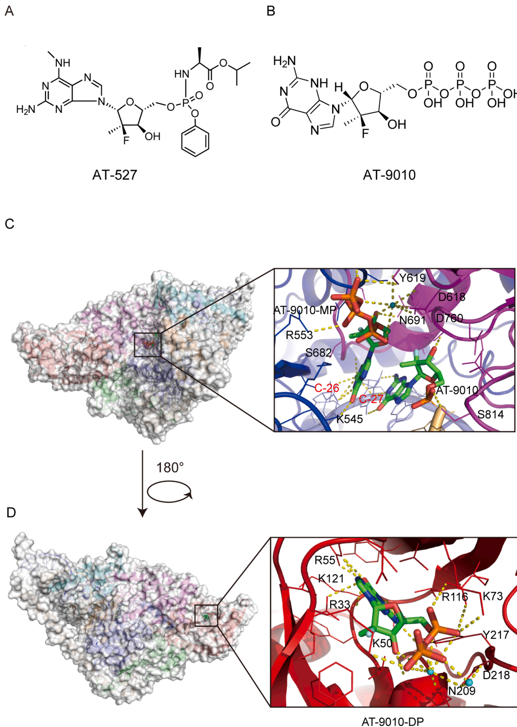
Fig. 7. Cryo-EM structure of AT-9010 bound to the RdRp complex of SARS-CoV-2 (PDB ID:7ED5) (A) Chemical structures of AT-527 and its active triphosphate form AT-9010. (B and C) Overall view of three AT-9010 molecules bound polymerase complex of SARS-CoV-2 and close up of RdRp catalytic site following AT-9010 incorporation (B) and binding of AT-9010 diphosphate (AT-9010-DP) in the NiRAN domain (C). In the RdRp active site, one AT-9010 monophosphate (AT-9010-MP) is incorporated at (+1) position, with an incoming AT-9010 occupying the (-1) position. In the NiRAN domain, AT-9010 is bound in its diphosphate form (AT-9010-DP). The potential polar contacts are shown as yellow dashed lines. The protein and RNA are shown in cartoons with the key residues involved in AT-9010 interaction shown in lines and labeled in black and red, respectively. AT-9010 are shown as stick models.
