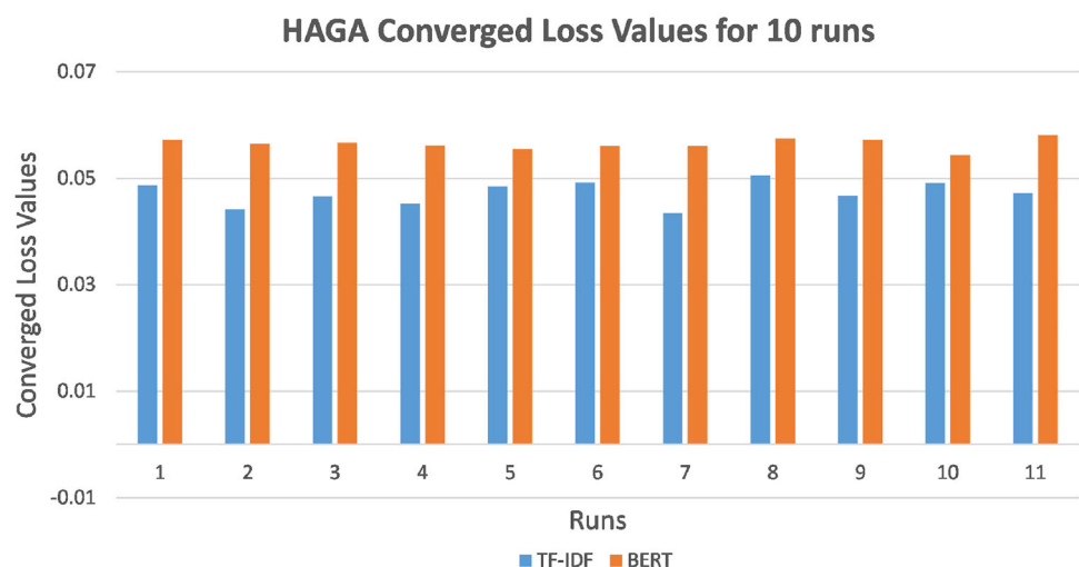
Fig. 5 Converged loss values for ten runs of HAGA
