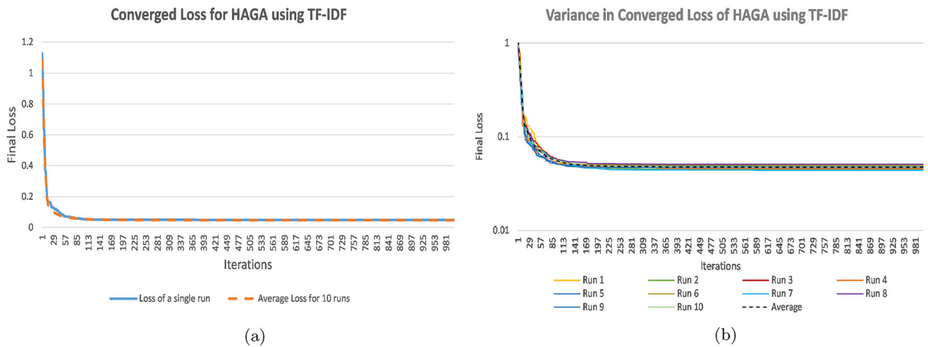
Fig. 7 Convergence of the HAGA in EHHR_{TFIDF} a Final Loss for single run compared to the final loss of average of ten runs, b Variation in final loss for ten different runs and the final loss of average of ten runs
