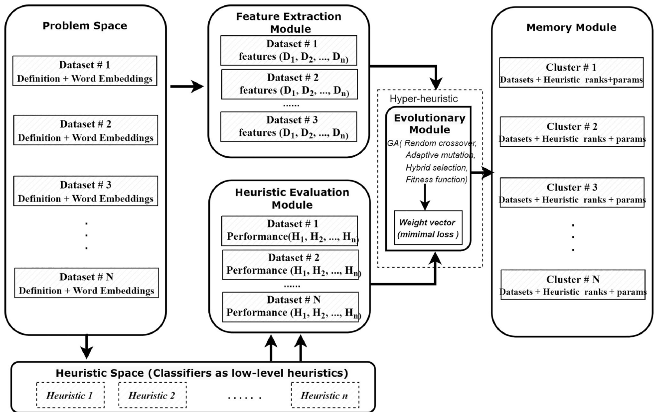
Fig. 2 The proposed framework of EHHR for short-text data
