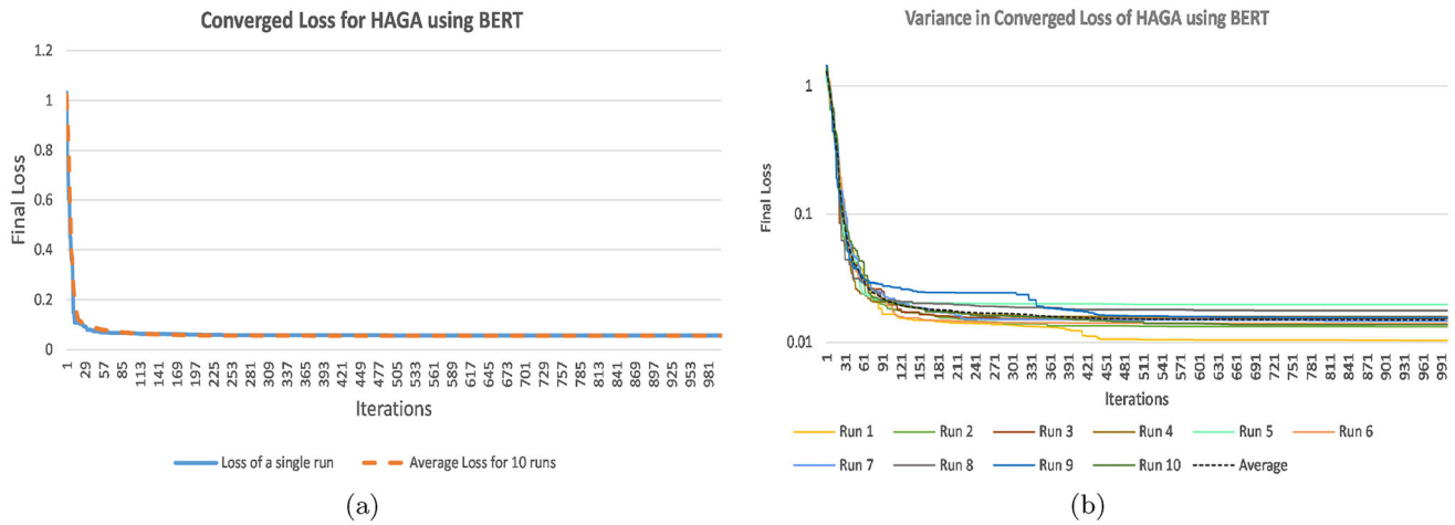
Fig. 6 Convergence of the HAGA in EHHR_{BERT} a Final Loss for single run compared to the final loss of average of ten runs, b Variation in final loss for ten different runs and the final loss of average of ten runs
