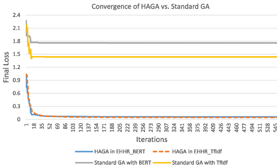
Fig. 9 Comparison of HAGA with Standard GA for Converged Loss iterations
