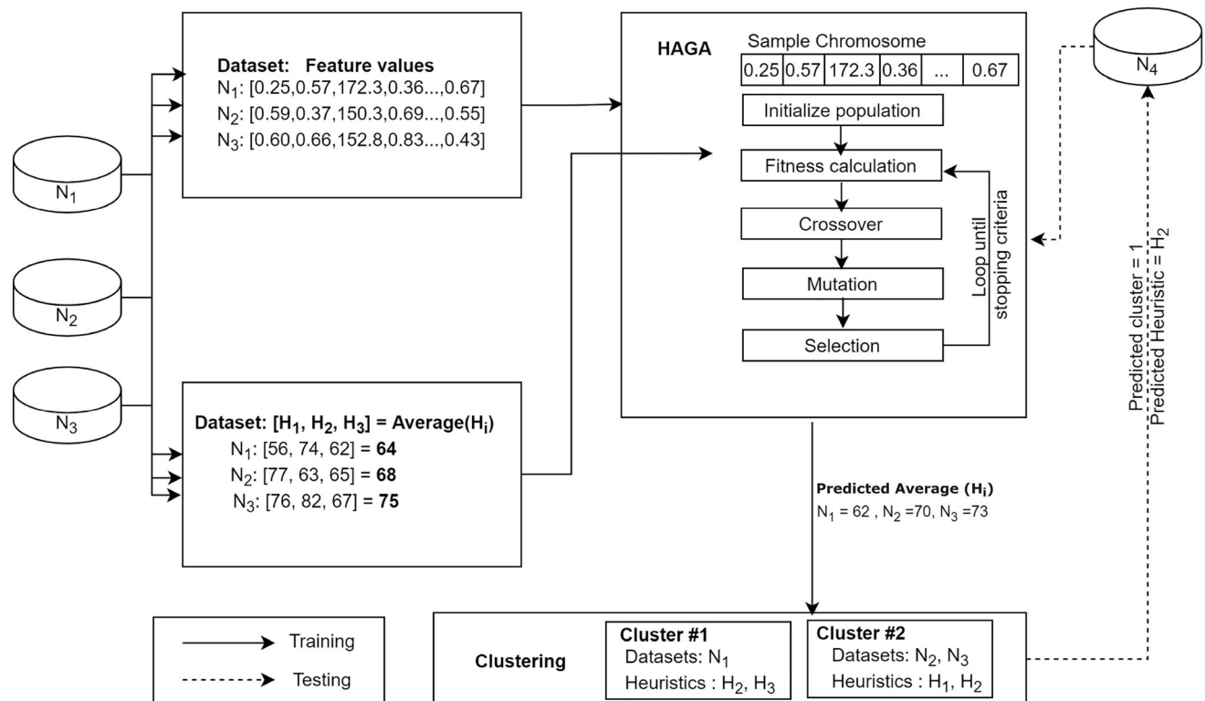
Fig. 4 An example of training and testing in EHHR
