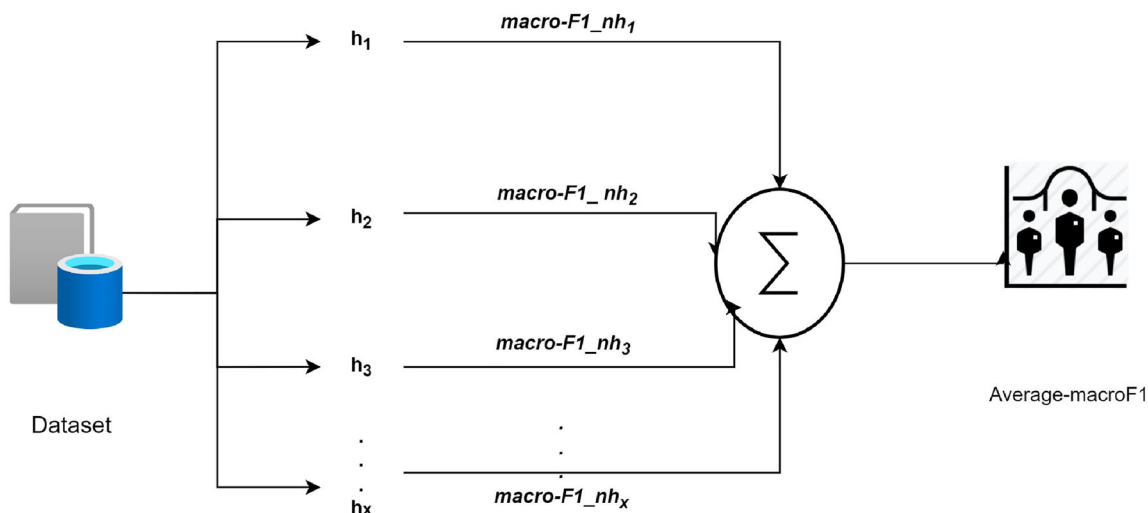
Fig. 3 The heuristic evaluation process in EHR resulting in computation of actual performance in terms of average macro-F1 for each dataset n \in N
