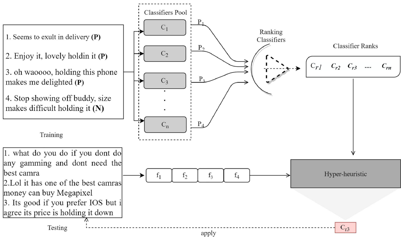
Fig. 1 Handling of classifier selection problem through Hyper-heuristic. C_{ri} is classifier's rank, f_i are dataset-level features. P_i is the performance of classifier C_i . C_{r3} is the best-predicted classifier for testing the dataset
