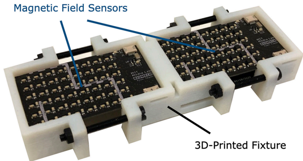
Figure 6: Magnetic Field Sensing Array.
