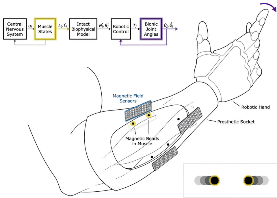
Figure 1: Free-Space Control of a Robotic Prosthesis via Muscle Magnetometry.
