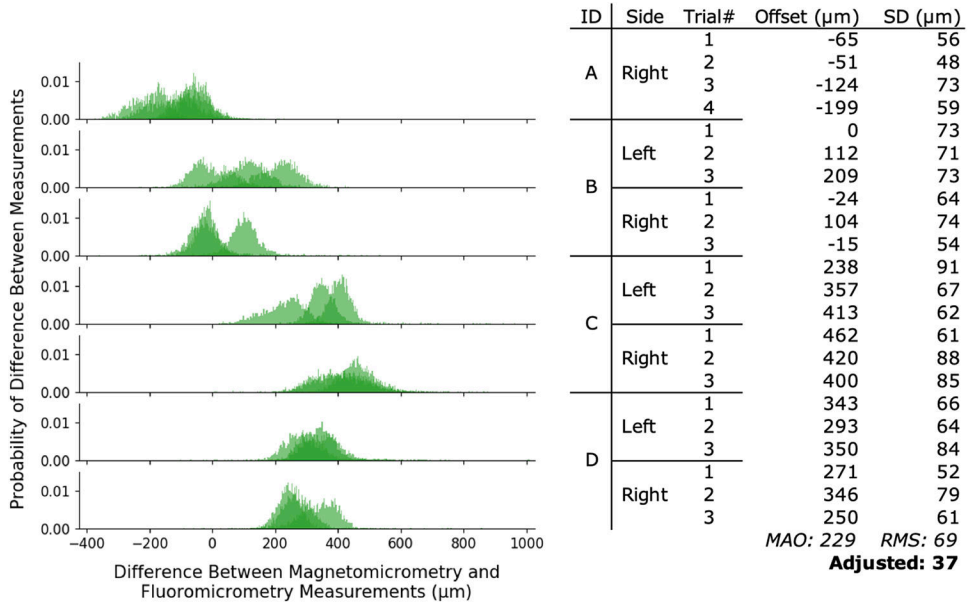
Figure 3: Difference Between Magnetomicrometry and Fluoromicrometry Gastrocnemius Frequency Sweep Measurements, in Micrometers.
