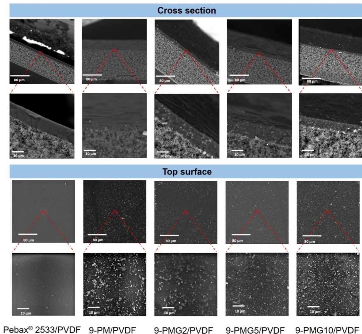
Fig. 7 SEM images of cross-section and surface of the pristine Pebax® 2533 membrane; MMMs with 9.1 wt% of MIL-101 (Fe); MIL-GO-2; MIL-GO-5; and MIL-GO-10, respectively.
