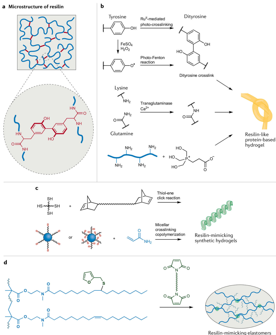
Fig. 2 | Chemical approaches in the design of resilin-mimicking materials.
