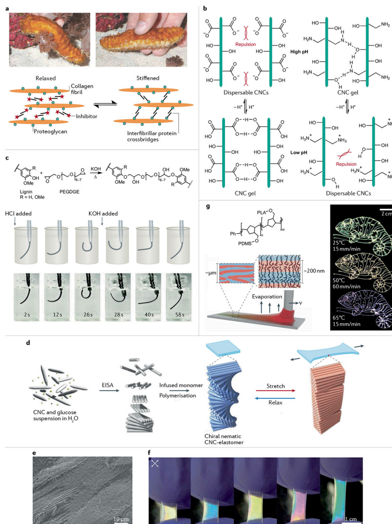
Fig. 4 | Preparation and chemistry of biomimetic stimulus-responsive polymer composites. a | Sea cucumbers can switch between relaxed and stiffened states because of their mutable collagenous tissue 9 . In simple terms, the stiffness-changing behaviour involves spindle-shaped collagen fibrils, which are discontinuous parallel aggregates 102 . Proteoglycans bind proteins such as styparin and tensilin, which bridge the fibrils. b | Amine- or carboxy-functionalized cellulose nanocrystal (CNC) suspensions have a pH-dependent stiffness that depends on attractive hydrogen bonds or electrostatic repulsions 105 . c | Lignin-based pH-responsive reversible actuators 114 . d | A stretchable chiral nematic CNC-elastomer composite can be prepared by evaporation-induced self-assembly (EISA) 122 . e | A cross-section scanning electron micrograph of the CNC-elastomer film shows periodic structures. f | Photographs of CNC-elastomer samples viewed under crossed polarizers while stretched. g | Direct-write chameleon patterns can be generated under constant 3D printing conditions 143 . Printing speed v and substrate temperature can control on-the-fly tuning of photonic properties. PDMS, poly(dimethylsiloxane); PEGDGE, poly(ethylene glycol) diglycidyl ether; PLA, poly(lactic acid). Part a adapted with permission from REF. 9 , AAAS and REF. 102 , Springer Nature Limited. Part b adapted with permission from REF. 105 ,
