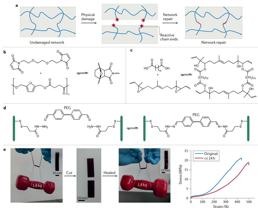
Fig. 5 | Biobased elastomers and hydrogels with dynamic chemical networks can self-heal.
