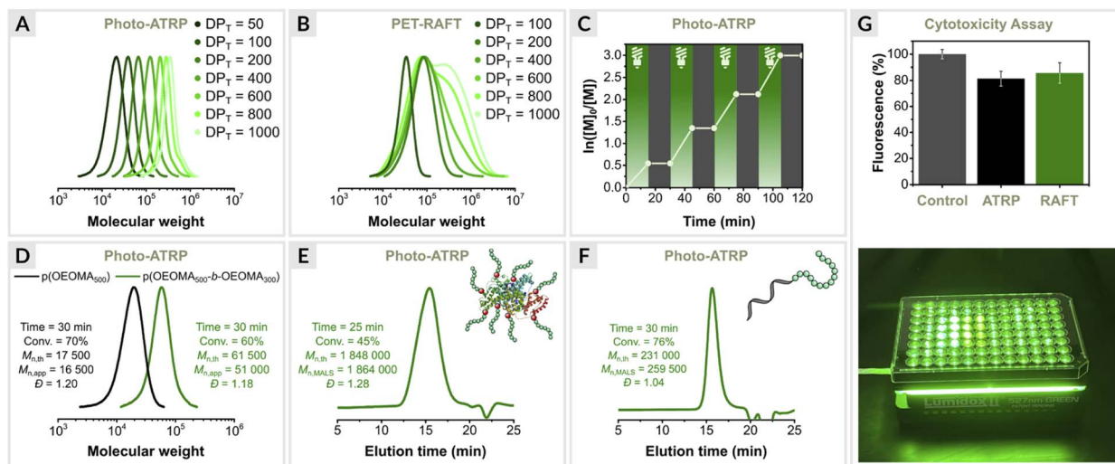
Fig. 4 Varying targeted degrees of polymerization, (A) EY/Cu mediated photo-ATRP, (B) EY-catalyzed PET-RAFT polymerization, (C) Temporal control, (D) Chain extension, (E) BSA-p(OEOMA 500 ), (F) DNA-p(OEOMA 500 ). (G) Comparison of the cytocompatibility of photo-ATRP with PET-RAFT polymerization.
