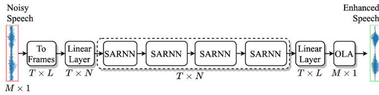
Fig. 5: The proposed SARNN for time-domain speech enhancement.
