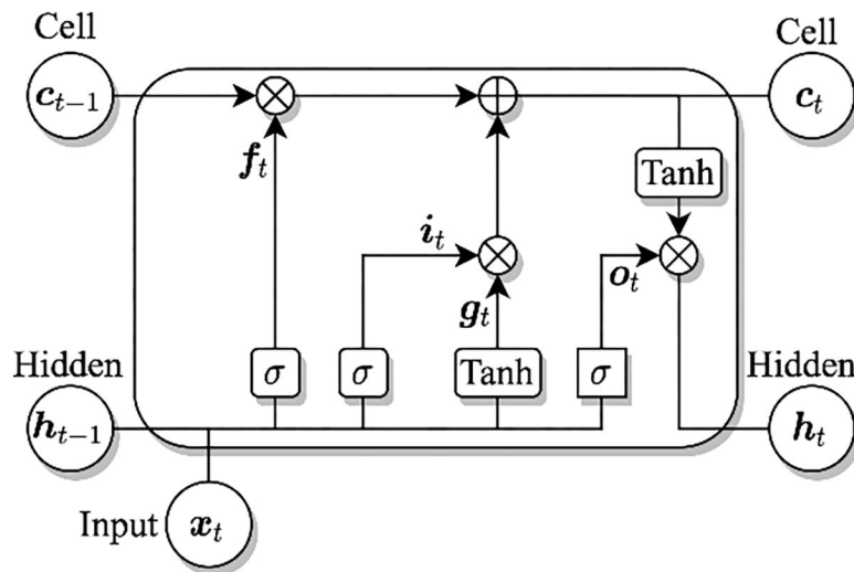
Fig. 2: A diagram of an LSTM with three gates. Symbol \otimes denotes elementwise multiplication.
