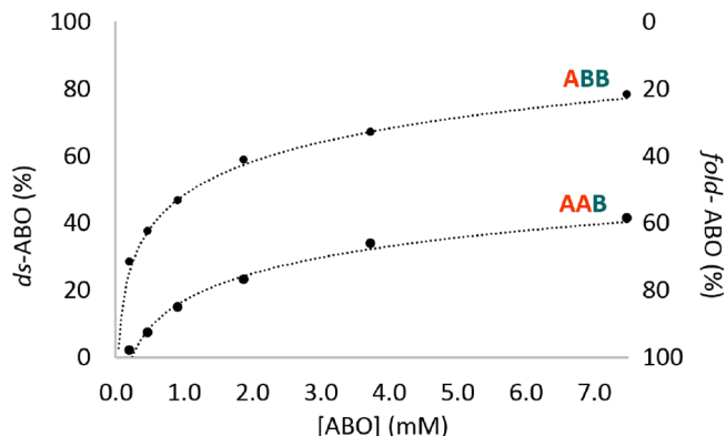
Figure 4. Concentration dependence of fold - vs ds -ABO in \text{CDCl}_3 with 2 mM TFA.
