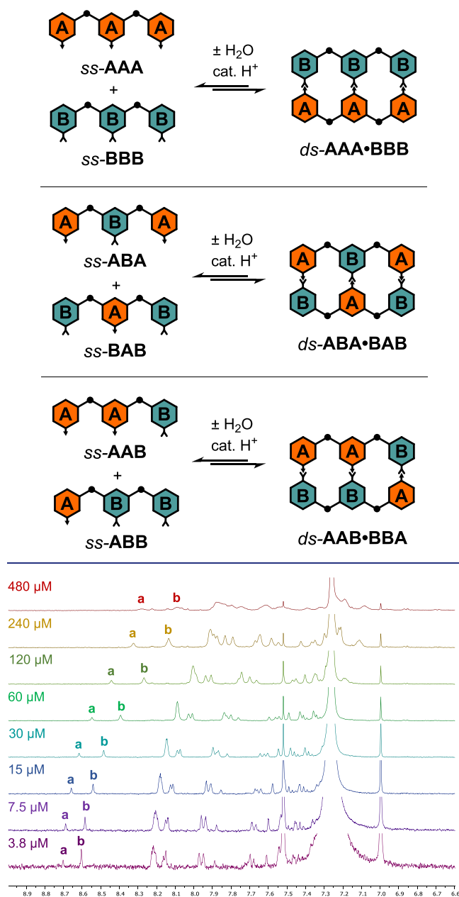
Figure 7. Portion of the ^1\text{H} NMR spectra of ds\text{-AAA}\cdot\text{BBB} in \text{CDCl}_3 at rt over a dilution series from 480\ \mu\text{M} to 3.8\ \mu\text{M} . Relevant ^1\text{H} resonances labeled: (a) 1H imine CHN from internal base pair and (b) 2H imine CHN from terminal base pairs.
