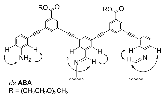
Figure 3. Key ^1\text{H} – ^1\text{H} ROSEY correlations observed for ds -ABA. As ds -ABA is C_2 symmetric, the other strand is magnetically equivalent to the half that is shown.
