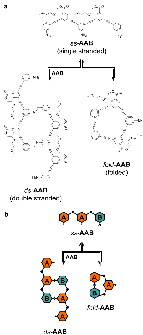
a (a) Skeletal structures of ss -, ds -, and fold -AAB. (b) Cartoon structures of ss -, ds -, and fold -AAB.
