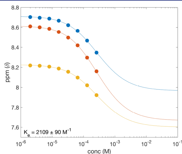
Figure 8. Concentration dependence of the ^1\text{H} NMR chemical shift of ds\text{-AAB}\cdot\text{BBA} in \text{CDCl}_3 at rt for three resonances: blue, the internal imine (NHC); red, the terminal imines (NHC); and yellow, the aromatic protons meta to the ester functional groups. Curves represent the line of best fit to the equal K model of indefinite association.
