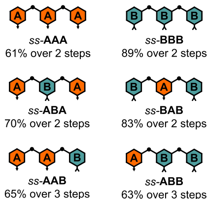
Figure 1. ss -ABO trimers. Isolated yields over the number of steps indicated.
