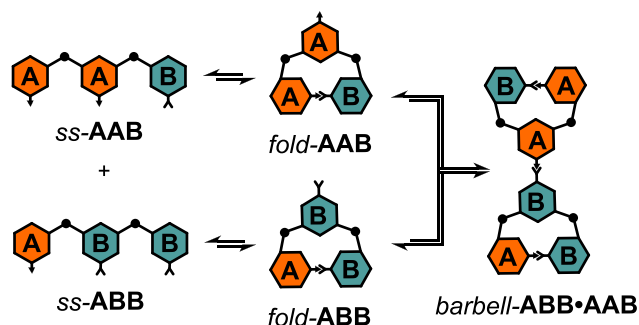
Scheme 5. Formation of barbell -AAB·BBA via the Condensation of fold -AAB and fold -ABB
