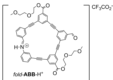
Figure 6. Structure of fold-ABB-H + .
