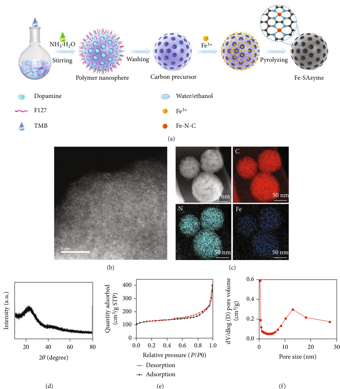
FIGURE 1: (a) Schematic illustration of Fe SAZ synthesis. (b) AC HAADF-STEM image of Fe SAZs. (c) HAADF-STEM image and corresponding EDS mapping of Fe SAZs. (d) XRD pattern of the Fe SAZs. (e) N_2 adsorption and desorption curves. (f) Pore size distributions for Fe SAZs.
