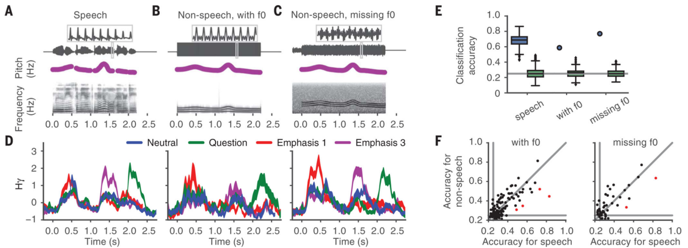
Fig. 3. Similar neural responses to intonation in speech and nonspeech contexts.
