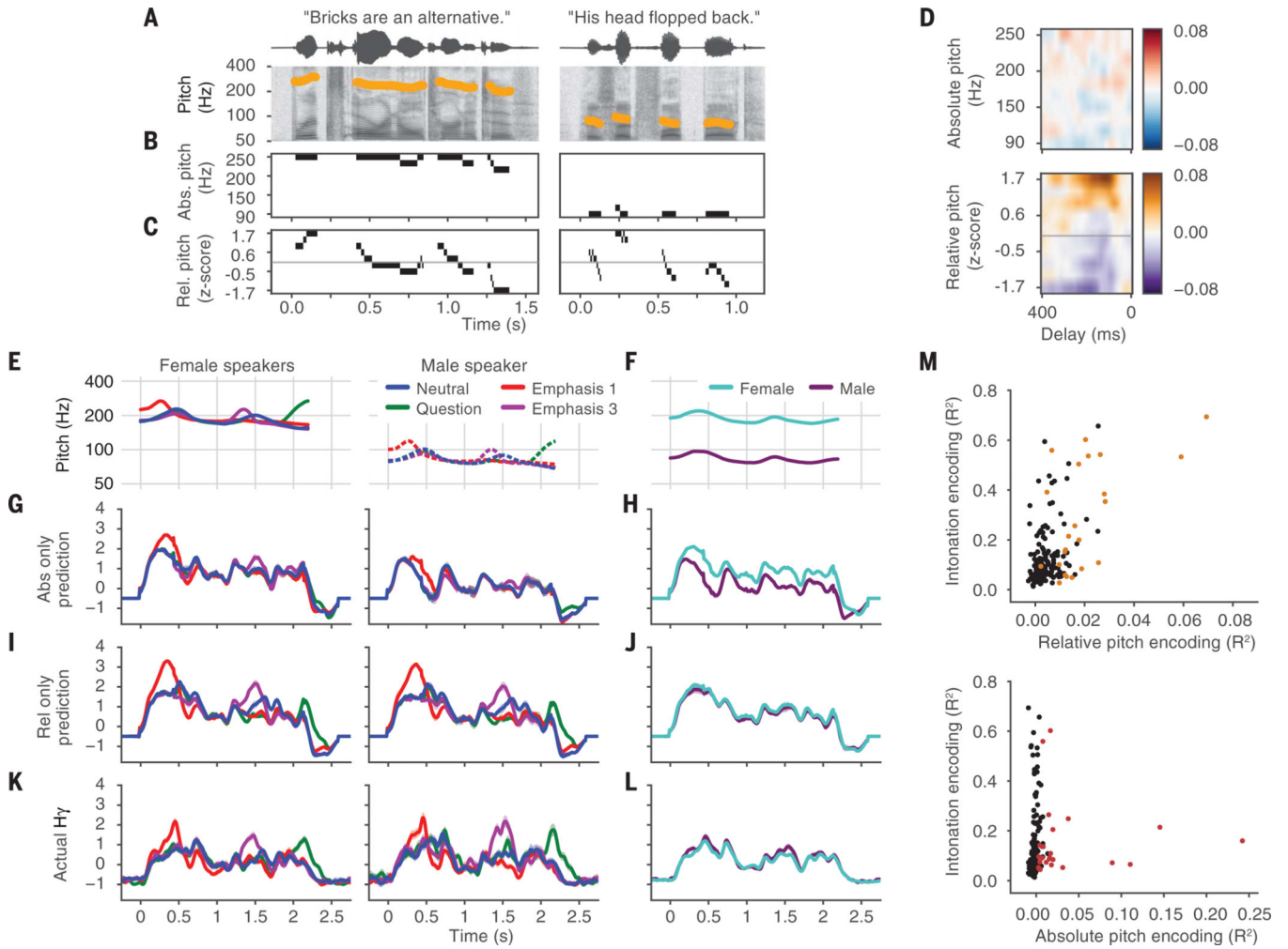
Fig. 4. Cortical representation of intonation relies on relative-pitch encoding, not absolute-pitch encoding.
