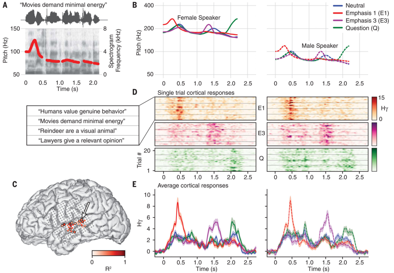
Fig. 1. Neural activity in the STG differentiates intonational pitch contours.
