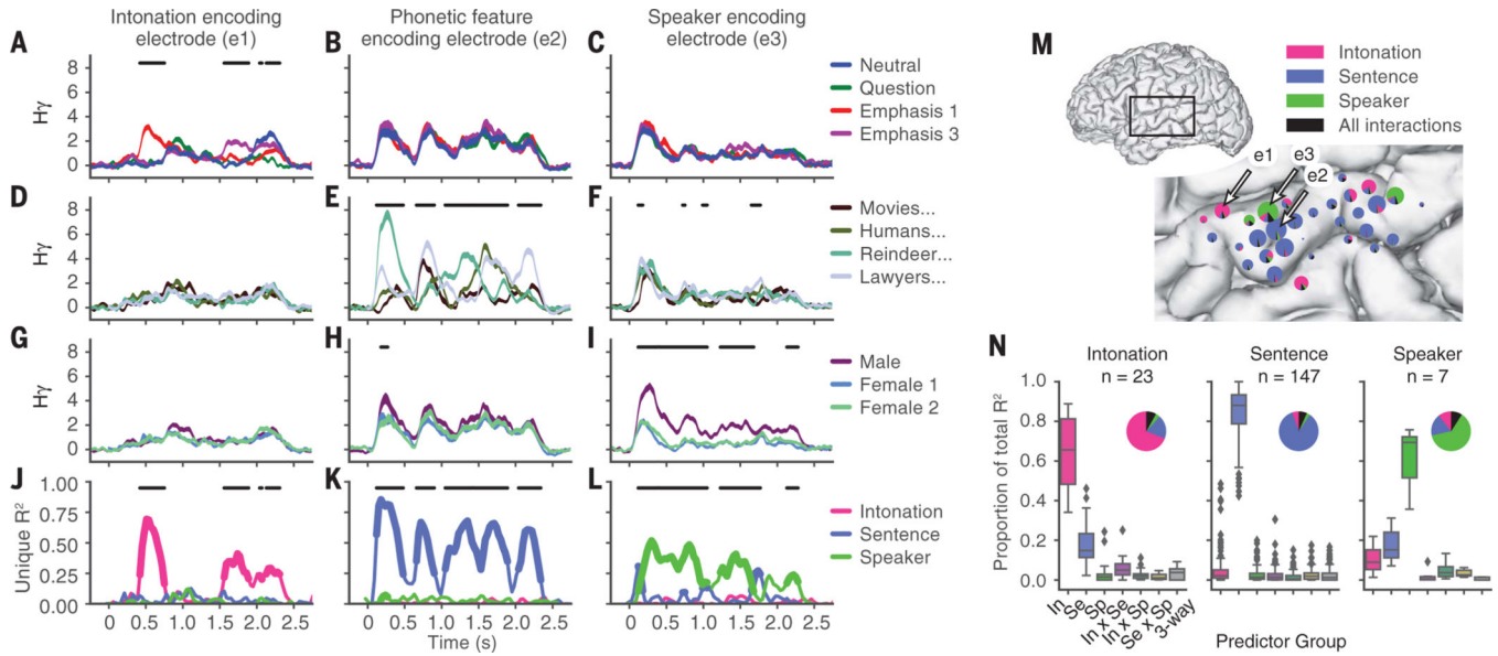
Fig. 2. Independent neural encoding of intonation, sentence, and speaker information at single electrodes.
