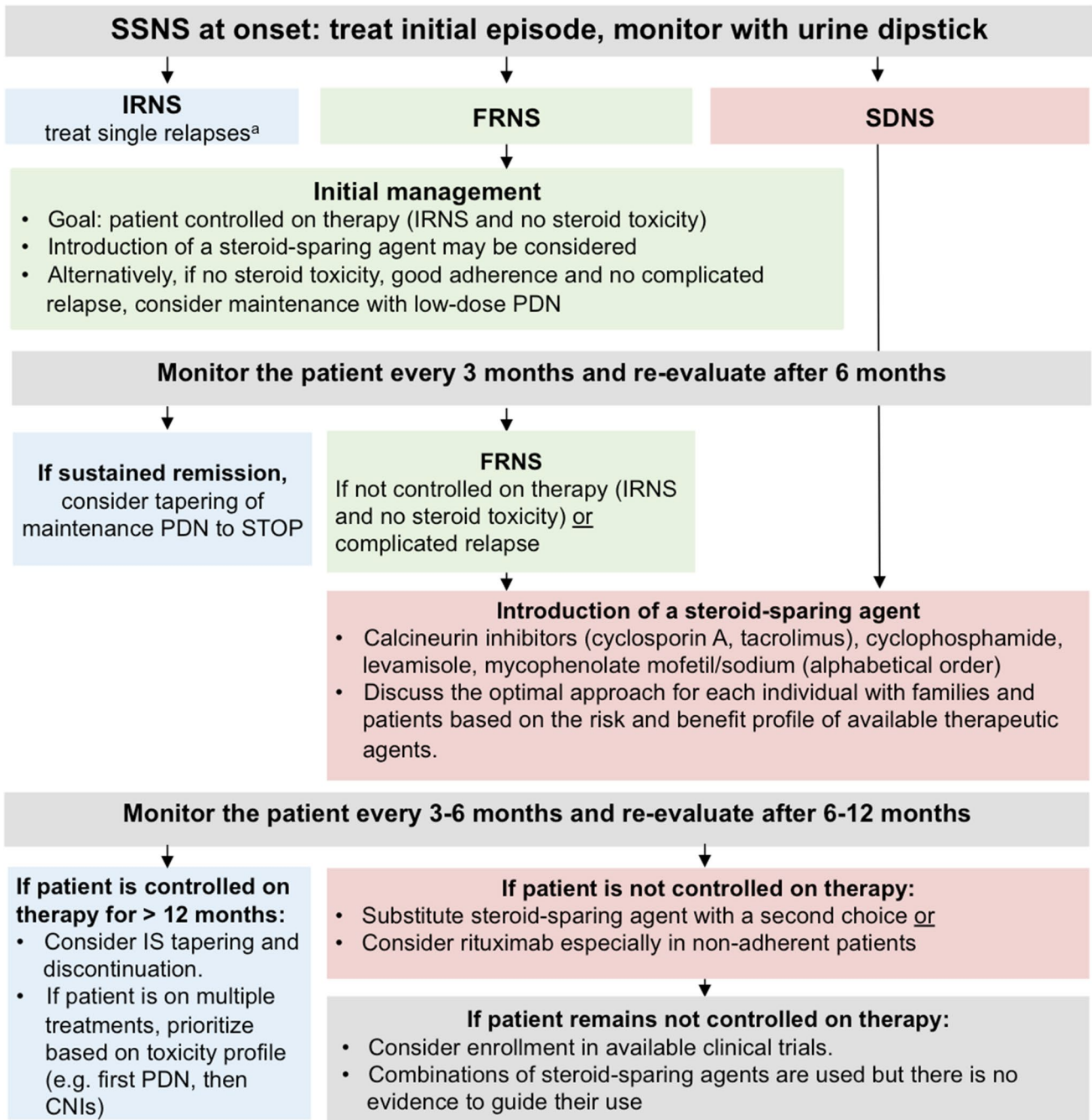
Fig. 3 Algorithm for management of children with SSNS. Details on the risk and benefit profile of the various steroid-sparing agents are given in Table 5 and Supplementary Table S6. IRNS infrequently relapsing nephrotic syndrome, FRNS frequently relapsing nephrotic
