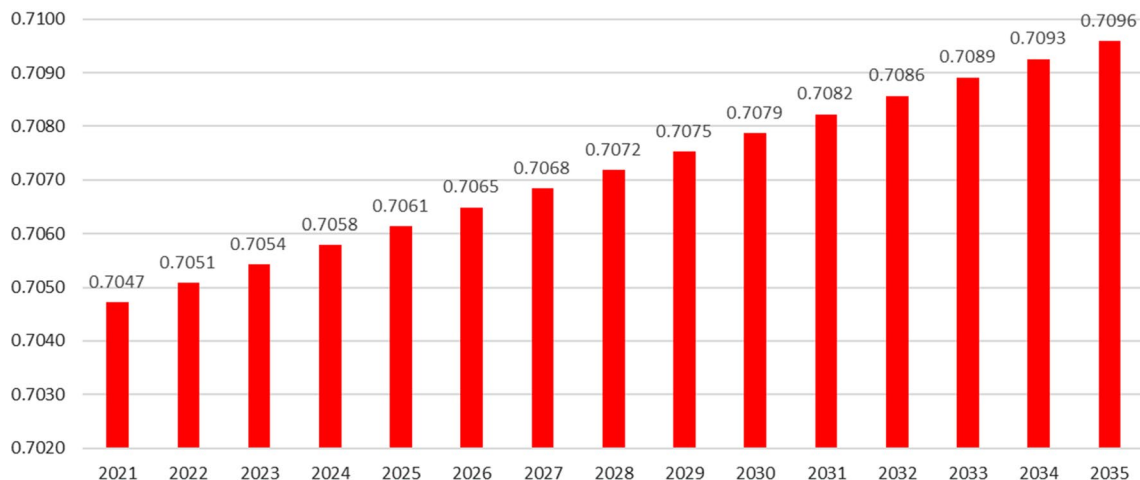
Fig. 9 Elasticity of substitution. The reduction of one unit of CO 2 causes a reduction of the utility level of country B by about 0.7096 in 2035. The elasticity of substitution increased annually by about 0.05% and over the analyzed time by about 0.69%. A growing utility gap can influence the political systems, if the consumers of country B perceive the utility decline as a welfare loss. First, it is well known that people compare themselves to others of the peer group [67]. Thus, the consumer of the developed country B might perceive the gap of international development negatively. Second, the perception might be even more negative, as the loss, which consumer of Country B faces, is more important than a gain with changes always being related to reference points according to the prospect theory by Kahneman and Tversky [68]
