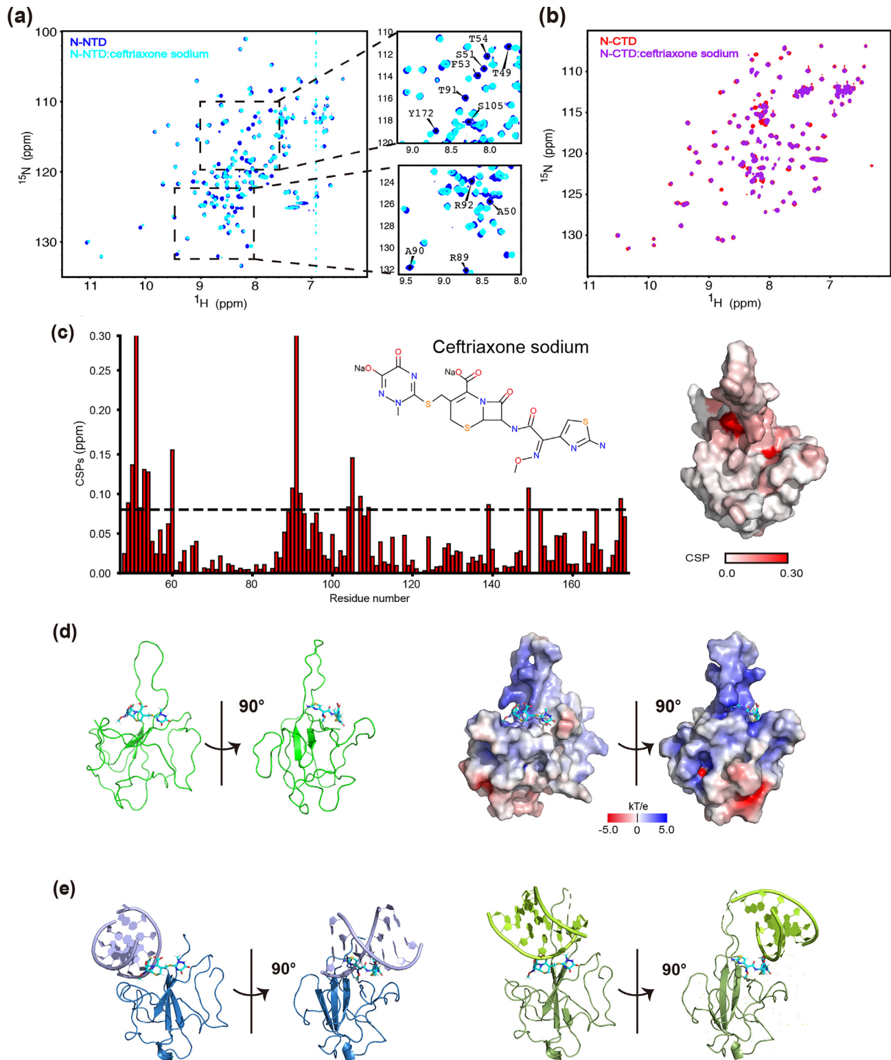
Fig. 3. NMR characterization of N-NTD/N-CTD and ceftriaxone sodium. (a) Superimposition of HSQC spectra of N-NTD in the absence (blue) and the presence of ceftriaxone sodium at a molar ratio (N-NTD: ceftriaxone sodium) of 1:25 (cyan). The assignments of the significantly perturbed residues are labeled on the right. (b) Superimposition of HSQC spectra of N-CTD in the absence (red) and the presence of ceftriaxone sodium at a molar ratio (N-CTD: ceftriaxone sodium) of 1:100 (purple). (c) Residue-specific chemical shift perturbations (CSPs) of N-NTD in the presence of ceftriaxone sodium at a molar ratio (N-NTD: ceftriaxone sodium) of 1:25. The significantly perturbed residues are defined as those with the CSP values at 1:25 > 0.08 ppm (average + STD) (dark dashed line). The surface representation of N-NTD is colored according to the CSP values in a white-to-red scale. Color intensities correlate with CSP values, with darker colors indicating larger values. (d) The structure of the NTD-ceftriaxone sodium complex with ceftriaxone sodium in sticks and N-NTD in cartoon (left) and electrostatic potential surface (right) are shown in two orientations. (e) Superimposition (based on \text{C}\alpha ) of ceftriaxone sodium-bound form and two dsRNA-bound forms of N-NTD reveals a similar binding interface. For the ceftriaxone sodium-bound form of N-NTD, only ceftriaxone sodium is shown.
