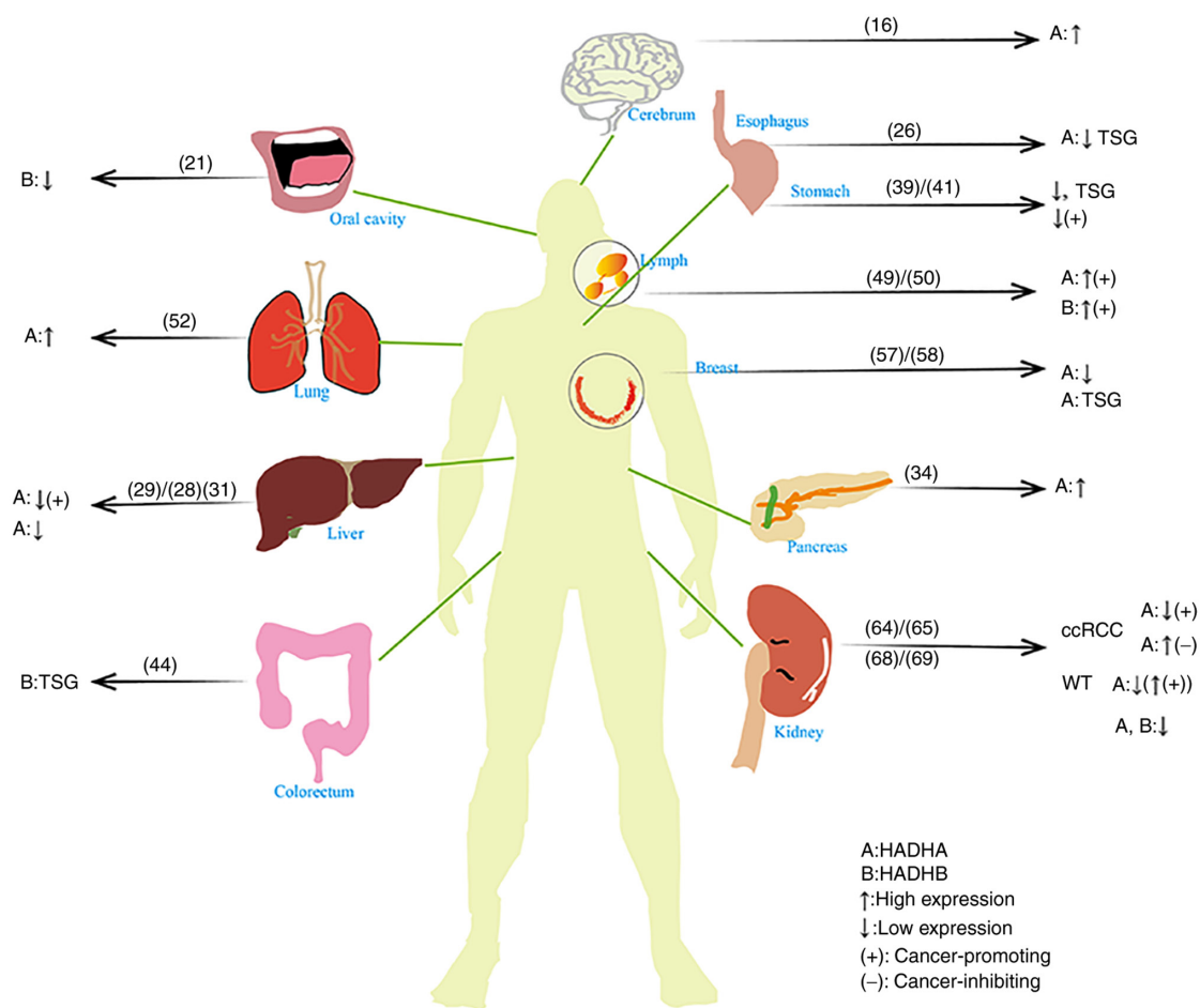
Figure 2. Expression of HADH in different organs. High HADHA expression inhibiting tumorigenesis or low HADHA expression promoting tumorigenesis: HCC, GC and ccRCC; High HADHA expression promoting tumorigenesis: Lymphoma. High HADHB expression promoting tumorigenesis: Lymphoma. A, HADHA; B, HADHB; ↑, high expression; ↓, low expression; (+), cancer-promoting; (-), cancer-inhibiting.
