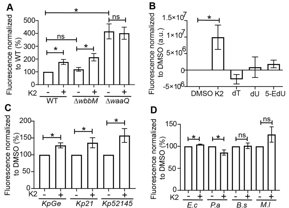
Fig 9. K2 treatment increases access of a hydrophobic probe to the bacterial membrane of K. pneumoniae . A. In order to assess the efficacy with which the LPS shielded the bacterial membrane, bacteria were exposed to the fluorescent probe 1-N-phenyl-naphthylamine (NPN), and fluorescence was recorded, providing a measure of the insertion of NPN in the bacterial membrane. The membrane of \Delta waaQ mutant K. pneumoniae was more accessible to NPN than that of WT and \Delta wbbM mutant. In K2-treated bacteria, access of NPN increased in WT and in \Delta wbbM but not in \Delta waaQ bacteria (mean \pm SEM; *: p < 0.05 ; Kruskal-Wallis test; N = 5 independent experiments). B. Three chemical analogs of K2 (dT = deoxythymidine, dU = deoxyuridine and 5-EdU = 5-Ethynyl-2'-deoxyuridine) were tested for their ability to increase the membrane accessibility of NPN. K2 was the only compound that increased significantly the accessibility of the outer membrane of K. pneumoniae to NPN (mean \pm SEM; *: p < 0.05 ; Kruskal-Wallis test; DMSO, K2: N = 6; and N = 5 independent experiments for the three analogs of K2). C, D. The effect of K2 was tested on three different strains of K. pneumoniae (KpGE, Kp21 and Kp52145) as well as Escherichia coli ( E.c ), Pseudomonas aeruginosa ( P.a ), Bacillus subtilis ( B.s ) and Micrococcus luteus ( M.l ). K2 increased NPN incorporation in K. pneumoniae , but exhibited little or no effect on other bacteria. (mean \pm SEM; *: p < 0.05 ; Mann-whitney test. N = 8 independent experiments).
