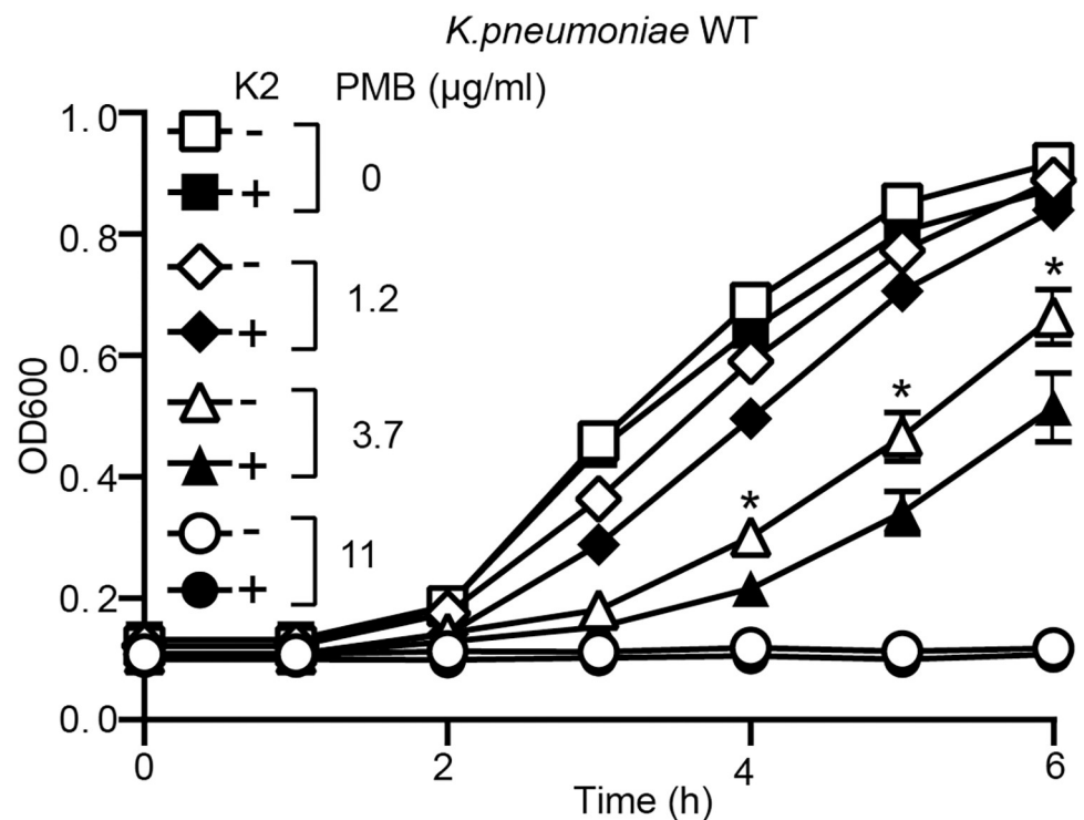
Fig 8. K2 increases the sensitivity of K. pneumoniae to polymyxin B. WT K. pneumoniae were grown overnight in the presence or absence of K2. The bacteria were then diluted and their growth was assessed for 6 h in the continued presence or absence of K2 and in the presence of increasing concentrations of polymyxin B (PMB: 0–11 \mu\text{g/ml} ). While exposure to K2 did not alter the growth of K. pneumoniae , it increased its sensitivity to polymyxin B as evidenced by a slower growth in the presence of 1.2 or 3.7 \mu\text{g/ml} of PMB (mean \pm SEM; *: p < 0.05 ; Mann-whitney test. PMB 3.7 \mu\text{g/ml} : N = 12 independent experiments).
