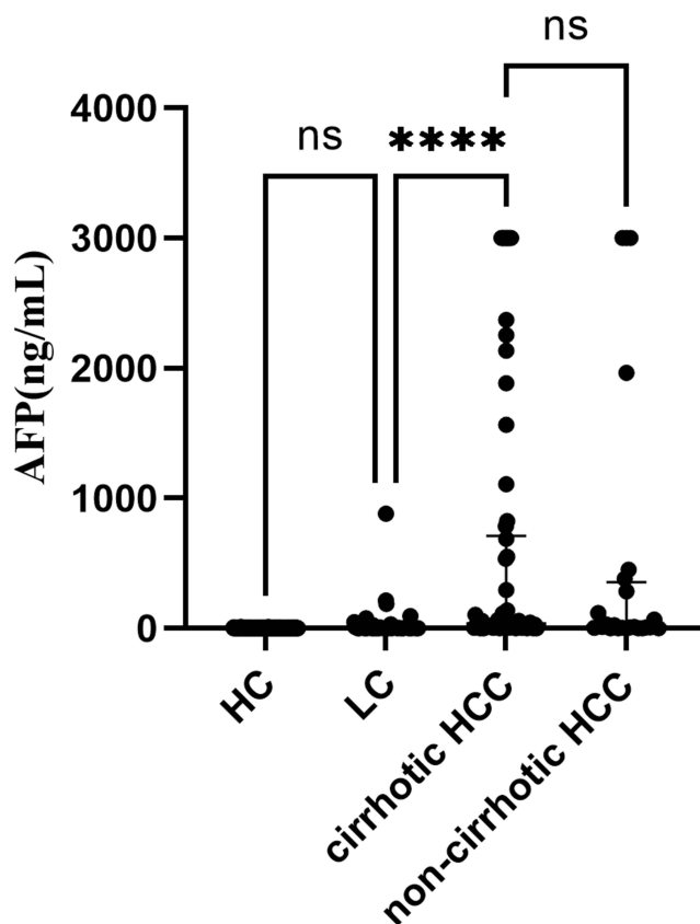
Figure 1 AFP levels in HC, LC, cirrhotic HCC and non-cirrhotic HCC. Participant numbers were respectively 152, 96, 62, 24 in HC, LC, cirrhotic HCC and non-cirrhotic HCC. NS means no significance with P > 0.05 , **** means P < 0.001 .
