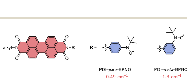
Fig. 3 Structures of the perylene diimide derivatives used for benchmarking and calculated values of J_{\text{TR}} using CASSCF/QD-NEVPT2.
