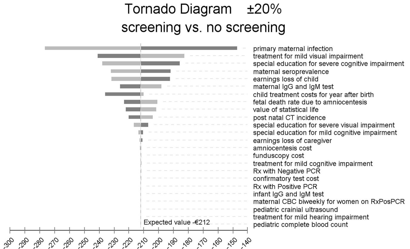
Fig 1. Tornado diagram.
