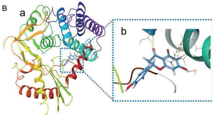
Fig. 4. Naringenin targets cGAS in HSCs. Mice with CCl 4 -induced fibrosis were treated with naringenin (100 mg/kg) for 8 weeks (3 times/week). (A) Fluorescence staining of HSC activation indicators α-SMA and cGAS in liver tissue sections. α-SMA and cGAS were coexpressed in liver tissues, and naringenin reduced the expression levels of α-SMA and cGAS in CCl 4 -induced liver fibrosis. Scale bar 20 μm. (B) Molecular docking of naringenin and cGAS using molecular modeling packages in the Maestro workstation. (A) cGAS, (B) naringenin, (C) Two-dimensional diagram after molecular docking. α-SMA, alpha smooth muscle actin; cGAS, cyclic guanosine monophosphate-adenosine monophosphate synthase.
