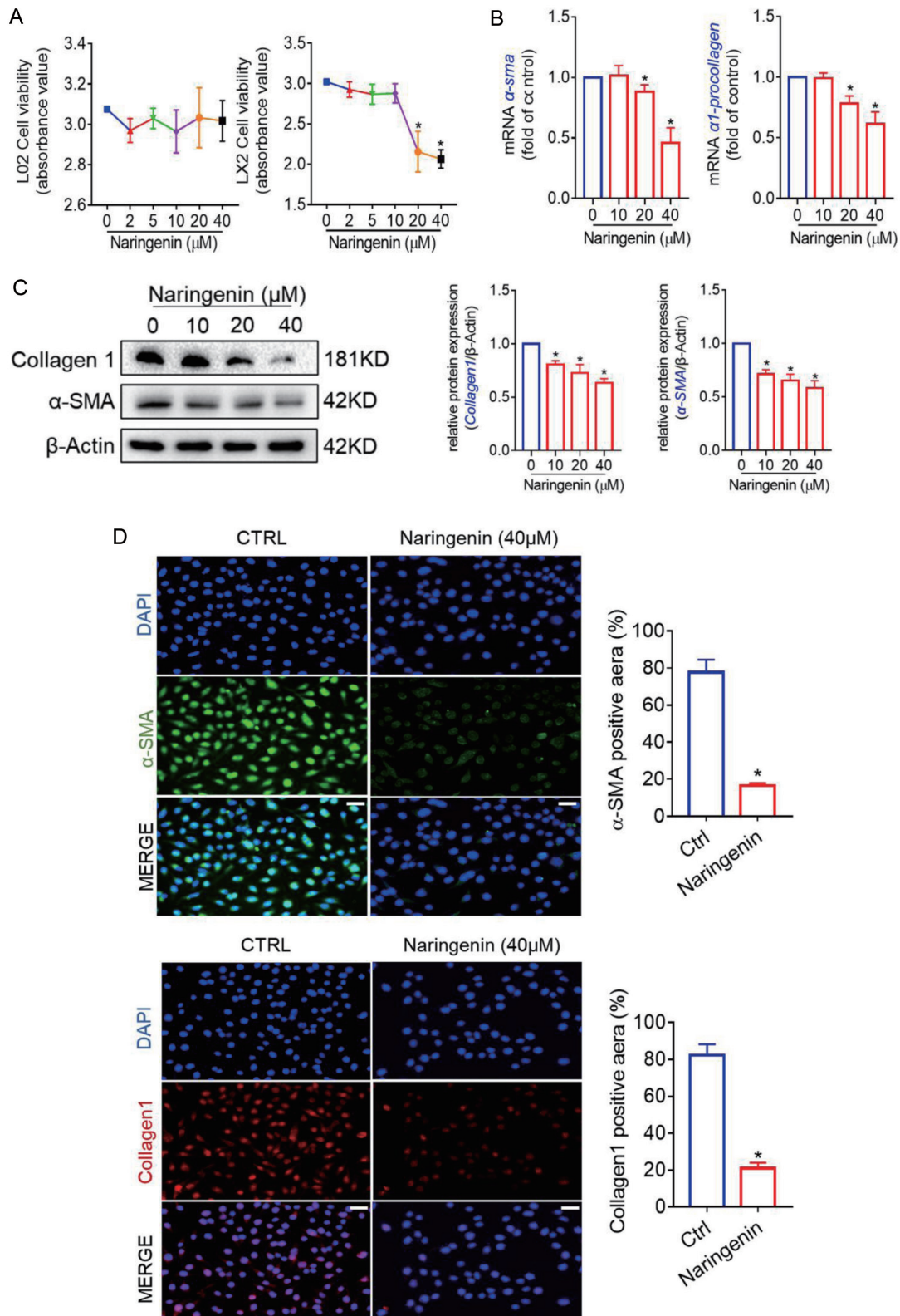
Fig. 5. Naringenin inhibits the activation of HSCs in vitro . HSC-LX2 were treated with naringenin for 24 h. (A) MTT assays showed that naringenin significant inhibited LX2 at 20 μM and had no effect on L02 cells. (B) Real-time PCR shows that naringenin inhibited expression of the LX2 activation indicators α-SMA and α1-procollagen in a dose-dependent manner. (C) WBs showed that naringenin dose-dependently reduced protein expression of α-SMA and collagen1 in LX2 cells, quantitative analysis, n=3 . * p<0.05 , versus naringenin (0 μM). (D) Immunofluorescence. Scale bar 20 μm. * p<0.05 , versus naringenin (0 μM). α-SMA, alpha smooth muscle actin.
