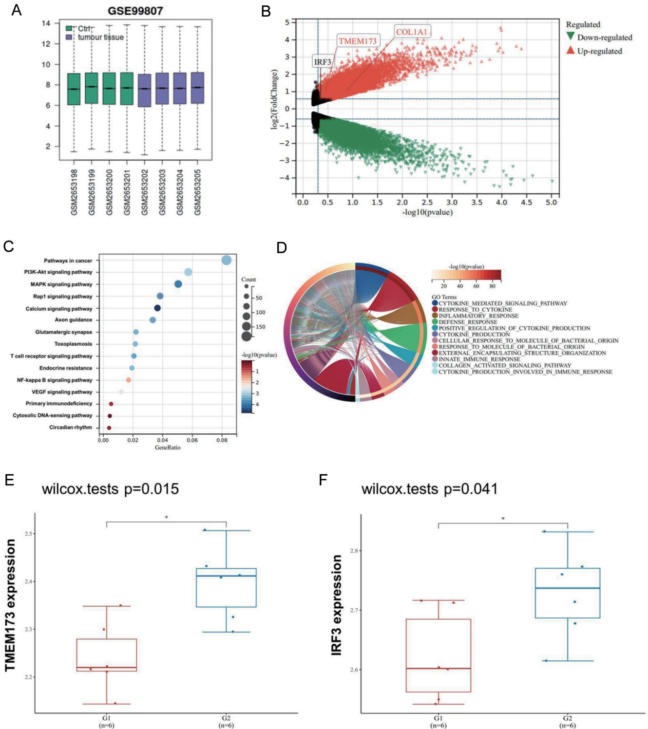
Fig. 1. TMEM173 (STING) and IRF3 are excessively expressed in liver fibrosis tissues from liver cancer patients. (A) The GSE number and sample quality for RNA microarray analysis of liver cancer tissue (tumor tissue, n=4 ) and normal adjacent tissue (ctrl, n=4 ) from GSE99807. (B) A volcano map derived from the differentially expressed genes (screening condition, p<0.05 ) between liver cancer tissue (tumor tissue, n=4 ) and normal adjacent tissue (ctrl, n=4 ) from GSE99807. (C) Using the differentially expressed genes between liver cancer tissue (tumor tissue, n=4 ) and normal adjacent tissue (ctrl, n=4 ) from GSE99807 to perform KEGG signal enrichment. (D) Using the differentially expressed genes in liver cancer tissue (tumor tissue, n=4 ) and normal adjacent tissue (ctrl, n=4 ) from GSE99807 to perform GOBP enrichment. (E and F) The expression distribution of TMEM173 and IRF3 genes in tissues (G1: normal, n=6 ; G2: liver fibrosis, n=6 ) from GSE33650, the upper left corner shows the significance p -value test method. COL1A1, collagen type I alpha 1 chain; STING, stimulator of interferon genes; IRF3, interferon regulatory factor 3.
