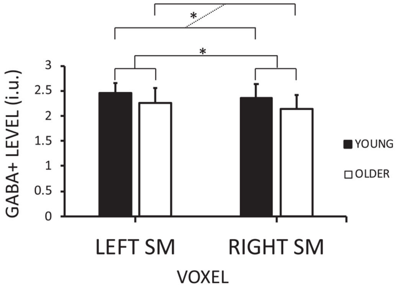
Fig. 3. GABA + levels per voxel [left and right sensorimotor (SM)] for both age groups (young and older adults). The dashed line emphasizes the age group (young vs. older) comparison. P < 0.05 is indicated by an asterisk.
