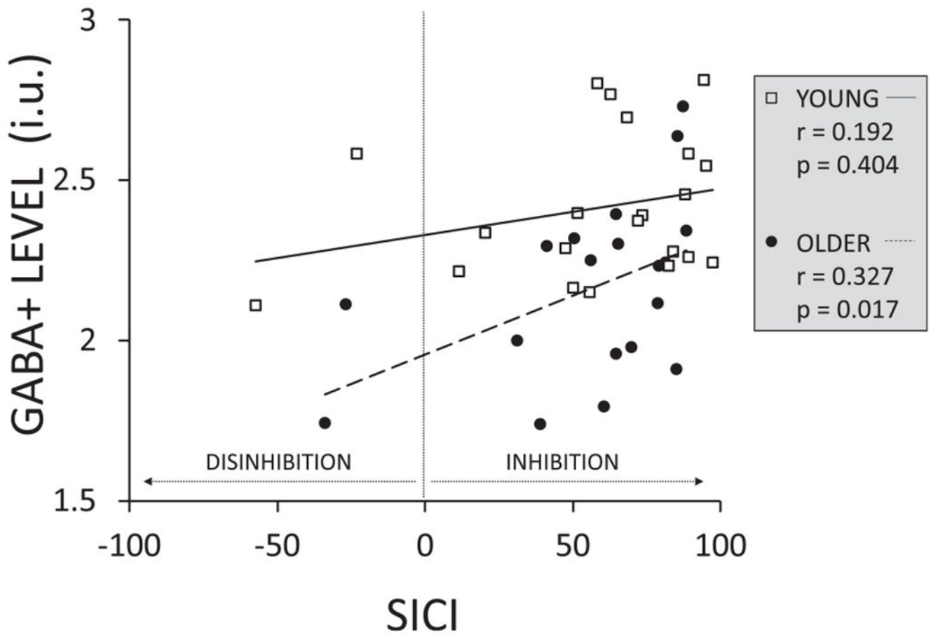
Fig. A.2. Exploratory correlations between GABA + level for the right sensorimotor (SM) voxel and short-interval intracortical inhibition (SICI) over the right M1 at the warning signal (preparation period) for older and younger adults. SICI was defined as: (1 - (\text{MEP}_{\text{pp}} / \text{MEP}_{\text{sp}})) * 100 .
