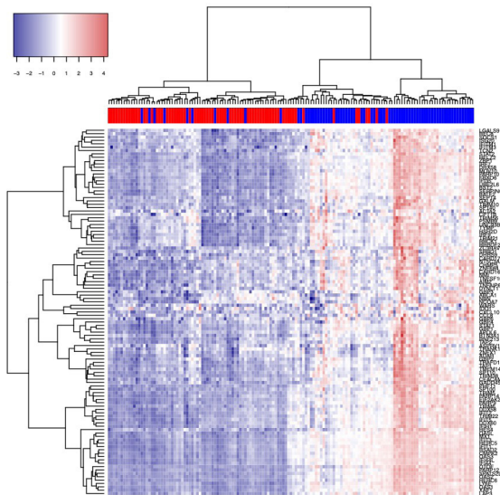
Figure 2 Heat map of expression of 110 interferon-stimulated genes 43 in SLE compared with HC. Subjects with SLE indicated by blue in the colour bar above the map, and HC indicated by red. ‘Pheatmap’ package V.1.0.12 1 is applied on DESeq2 normalised and variance stabilised gene expression values to create the heat map. 62 HC, healthy control.
