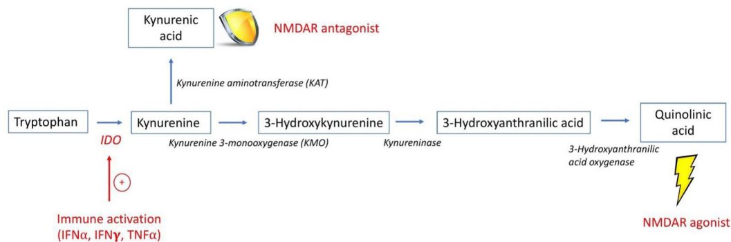
Figure 1 The kynurenine/tryptophan pathway. 1 This is a simplified schematic of the KYN/TRP pathway, highlighting the intermediates and enzymes involved in the production of QA and KA. The enzyme IDO1 is stimulated by inflammatory cytokines, such as IFN, that results in the breakdown of TRP into KYN. KYN may be further metabolised by KMO ultimately to QA, an NMDAR agonist, or by KAT to KA, an NMDAR antagonist. Since the enzyme KMO has higher affinity for KYN than KAT, metabolism proceeds preferentially towards the production of QA in the setting of inflammation. 2 26 61 IDO1, indolamine 2, 3-dioxygenase; IFN- \alpha , interferon alpha; IFN- \gamma , interferon gamma; KA, kynurenic acid; KMO, kynurenine 3-monooxygenase; NMDAR, N-methyl-D-aspartate receptor; QA, quinolinic acid; TNF- \alpha , tumour necrosis factor alpha.
