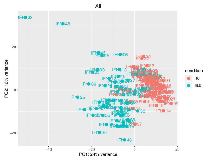
Figure 3 PCA of gene expression in SLE compared with HC. PCA conducted on DESeq2 normalised, and variance stabilised gene expression values, using the function prcomp in R V.3.5, 1 is displayed. The default top 500 most highly variant genes were selected. 63 HC, healthy control; PCA, principal component analysis.
