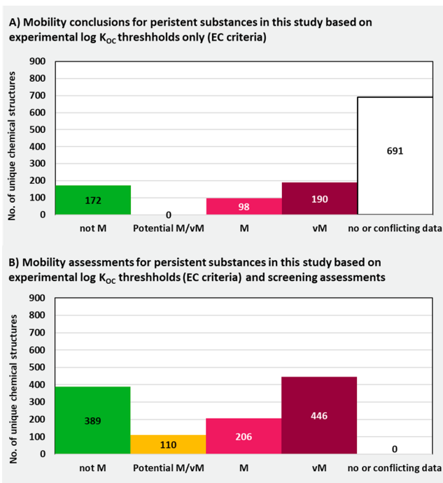
Figure 10. Mobility assessments of the substances considered in this study that were assessed as P, vP, and Potential P/vP++ using (A) the criteria proposed by the EC based on \log K_{OC} thresholds and (B) the additional screening thresholds based on \log K_{OW}/D_{OW} screening parameters in Figure 9.
