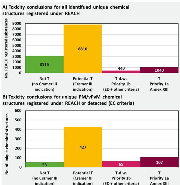
Figure 11. Distribution of toxicity assessments for (A) all identified unique chemical structures registered under REACH or transformation products thereof and (B) all identified persistent and mobile (PM) or very persistent and very mobile (vPvM) chemical structures registered under REACH or detected in the environment.
