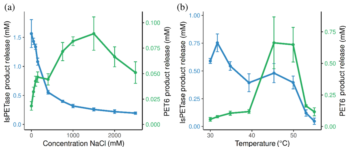
FIGURE 2 Activity of PET6 and IsPETase on PET at varying temperatures and salt concentrations. PET6 (green line) and IsPETase (blue line) were incubated for 18 hr at a concentration of 2 \mu M and 20 nM, respectively. (a) The effect of salt concentrations on the two enzymes varied between 0 and 2,500 mM (measured in 96-well reaction plates at 30°C). (b) Different incubation temperatures in the range of 30 and 55°C were tested (measured in coated PCR tubes) with the sodium chloride concentration fixed at 50 mM. PET, plastic polyethylene terephthalate
