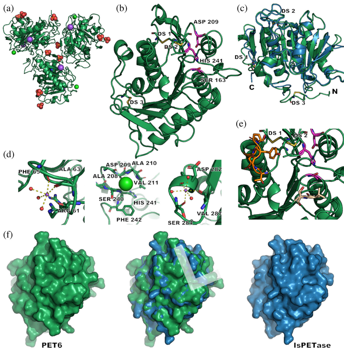
FIGURE 3 Crystal structure of PET6 (green) and comparison to IsPETase (blue). (a) Shows the asymmetric unit of the PET6 crystal structure (green, PDB ID 7Z6B ) containing three protein molecules; ions are depicted as colored spheres including phosphate (orange-red), sodium (purple), and chloride (neon green). (b) Displays a single chain, with the catalytic triad (Ser-His-Asp) highlighted in pink; the three disulfide bonds are labeled DS1-3. (c) Illustrates how the superimposed structures of PET6 and IsPETase ( 5XJH ) have only a few deviations in loops and termini. (d) Highlights ion binding with the two sodium ions (violet) being coordinated by three carbonyl oxygens and three water molecules, while chloride (neon green) is located in a small pocket. The positions of subsequent mutations are shown in (e) with the loop region (Ex-Loop) in dark orange and two residues for the double mutant VSTA in beige in proximity to the active site colored in pink. (f) Compares the surface of the two proteins with a focus on the putative substrate-binding site approximated as L shape in the superimposed structure.
