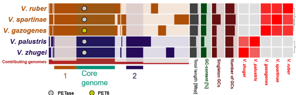
FIGURE 1 Pangenomic analysis of five PETase-containing Vibrio genomes. The analysis includes 6,651 GCs involving 19,117 individual gene calls. The five first tracks represent protein-coding GCs of individual genomes organized by ANI (red squares and cladogram) of the aligned fraction. Presence of a GC in a genome is indicated in dark colors, absence in light. The core genome of the analyzed Vibrio genomes is indicated in turquoise. Further GCs specific of each of the two clades are indicated in the color of the clade (1 and 2). The red track shows the number of genomes harboring a defined GC. Other genome statistics (from left to right: total length [0–6 Mbp], GC content [30–50%], number of singleton GCs [0–1,000] and number of GCs [0–5,000]) are indicated as additional bar charts on the right. The GCs containing PETase-coding genes are marked with a circle for each species. PET6 is highlighted in yellow. ANI, average nucleotide identity; GCs, gene clusters; PET, polyethylene terephthalate
