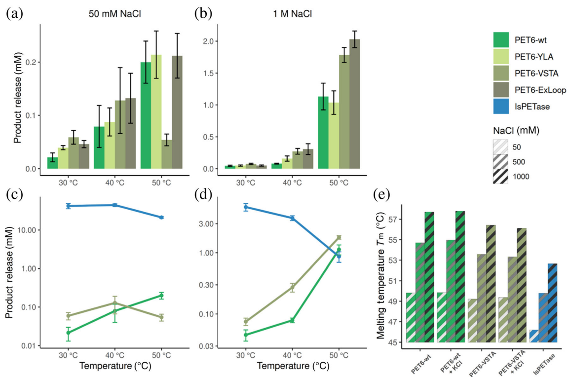
FIGURE 4 Performance of PET6 variants compared to IsPETase at varying temperatures and salt concentrations. PET6 variants (green) were used at a concentration of 2 \mu\text{M} and IsPETase (blue) at 200 nM and incubated for 18 hr. Therefore, the total product release of IsPETase was extrapolated by a factor of 10 to obtain comparable results within the activity experiments (a–d). The performance of the PET6 variants at different temperatures is compared in (a) at 50 mM and (b) at 1 M salt. The same data is shown in (c) and (d) for PET6-wt and PET6-VSTA with IsPETase for comparison; therefore, the y-axis is log 10 scaled to account for strongly varying performance levels. (e) Shows the analysis of T_m for PET6-wt, PET6-VSTA, and IsPETase at varying salt concentrations with DSC. The T_m of the enzymes was determined at 50, 500, and 1,000 mM NaCl as indicated in the hatching; the two PET6 variants were further characterized under the same conditions with additional 10 mM KCl. DSC, differential scanning calorimetry
