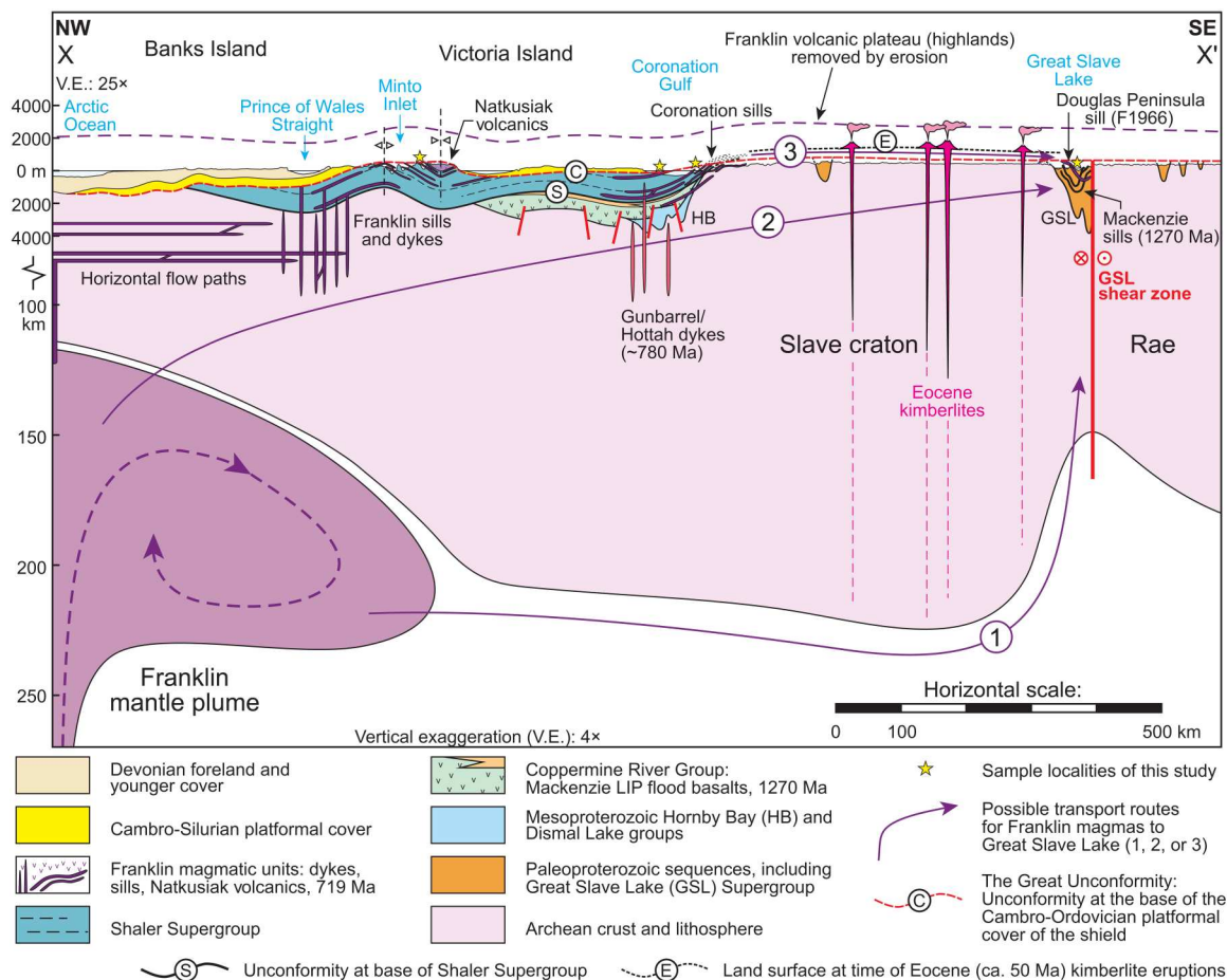
Fig. 2. Schematic cross section of the Franklin LIP and starting plume head, and surrounding geological units. The section illustrates the emplacement of the Franklin LIP and three possible paths for sill emplacement in the Great Slave Lake area. Victoria Island sills and dykes may have similarly been emplaced via horizontal flow paths through the lithosphere. Location of cross section X-X' is indicated in Fig. 1A. Dashed purple line depicts an estimate of the original Franklin LIP volcanic plateau thickness before erosion. Modern elevation on the y axis. Reconstructed paleosurfaces are positioned relative to the modern topography and do not indicate absolute paleoelevations at past times. NW, northwest; SE, southeast.
